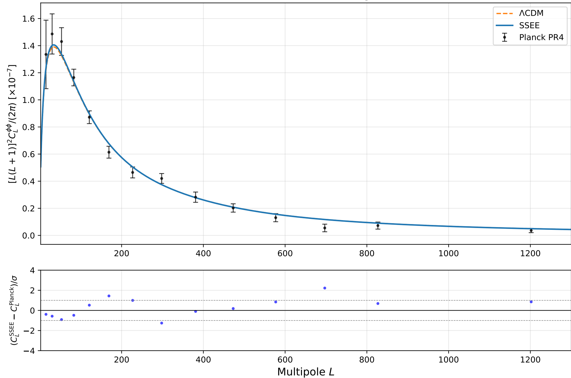
SSEE vs Planck PR4: CMB Lensing Potential
