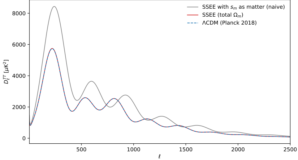
Figure 1: CMB TT power spectrum from CLASS. Blue dashed : \Lambda CDM Planck 2018. Red solid : SSEE with the full \omega_m -direct canonical matter density \Omega_{m,\text{CMB}} = 0.308881 ( w_0 = -0.839950 , w_a = -0.669975 ) — peaks at \ell = 220, 536, 813 , agreeing with \Lambda CDM to within \Delta\ell \leq 1 (RMS = 0.18%). Grey : the SSEE dynamical-only run ( \Omega_{m,\text{CMB}} = 0.160050 ); it produces peaks at \ell = 240, 596, 921 with RMS = 58.9% relative to \Lambda CDM, confirming that the full matter density (not the dynamical s_m = 0.160050 ) is needed to reproduce the acoustic scale.
