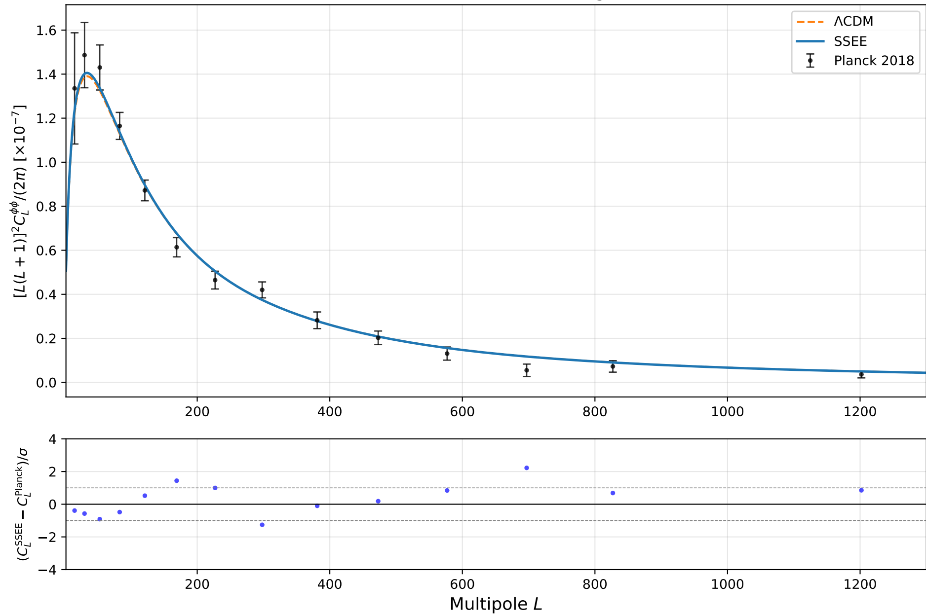
SSEE vs Planck 2018: CMB Lensing Potential
