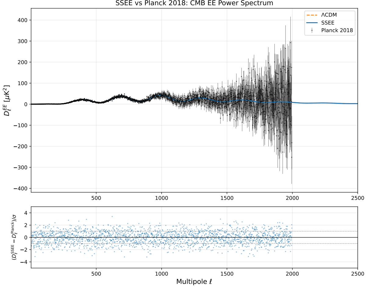
Figure 4: CMB EE polarization power spectrum D_\ell^{EE} [\mu\text{K}^2] . Blue: SSEE. Orange dashed: \Lambda\text{CDM} . Black points: Planck 2018 EE data.
