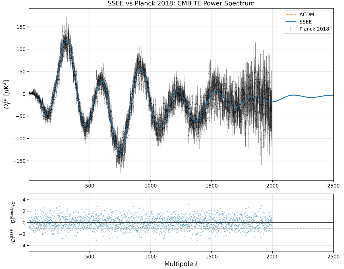
Figure 3: CMB TE cross-correlation power spectrum D_\ell^{TE} [\mu\text{K}^2] . Blue: SSEE. Orange dashed: \Lambda\text{CDM} Planck 2018 best-fit. Black points: Planck 2018 TE data. Lower panel: residuals normalised by \sigma_\ell .
