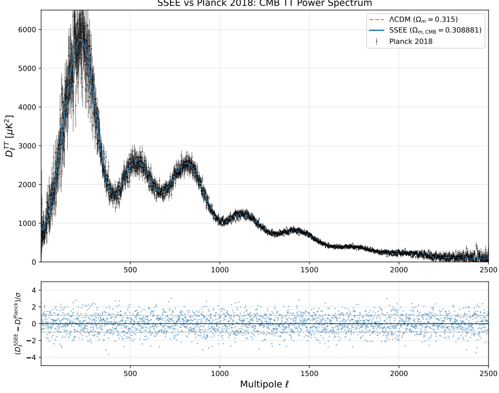
Figure 4: CMB temperature angular power spectrum computed with CLASS for the SSEE background and EFT functions (Eq. 9), compared against Planck 2018. With the dark-energy sector fixed by \varphi and \pi , SSEE reproduces the acoustic peaks at \ell = 220, 536, 813 at a quality indistinguishable from \Lambda CDM (Table 5). The full matter density is essential: replacing \Omega_m^{\text{cosm}} = 0.308881 with the equation-of-state number 1 + w_0 = 0.160050 moves the peaks to \ell = 240, 596, 921 .
