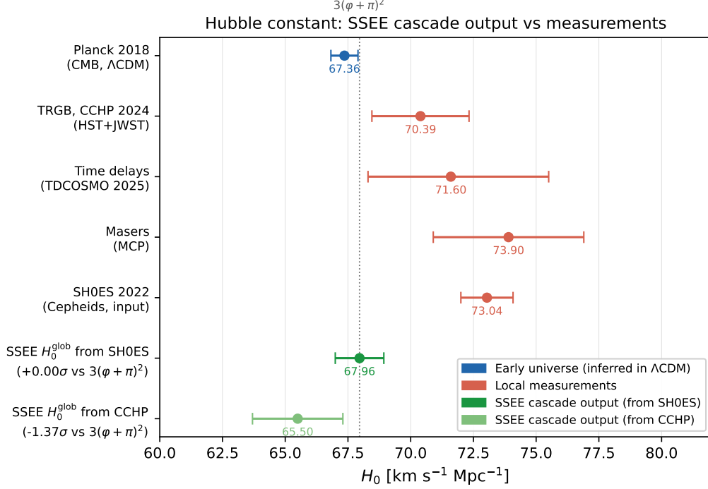
Figure 1: Hubble constant measurements: the early-universe inference (blue, within \Lambda CDM) and local measurements (red), each read from its publication, against the output of the SSEE cascade with the complete screening fraction (green). Run on SH0ES the cascade returns H_0^{\text{glob}} = 67.96214 km/s/Mpc; run on the TRGB value adopted by CCHP [Freedman et al., 2024] it returns 65.50 ( -1.37\sigma from 3(\varphi + \pi)^2 ), the control from the other side. Error bars show \pm 1\sigma .
