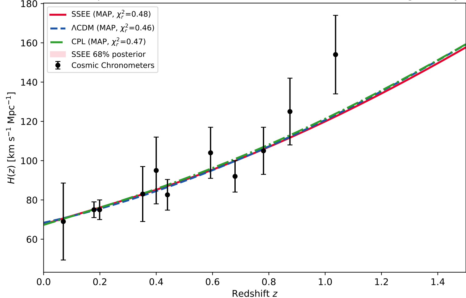
Posterior predictive check — H(z) (total matter \Omega_m = 0.308881 in geometry)
