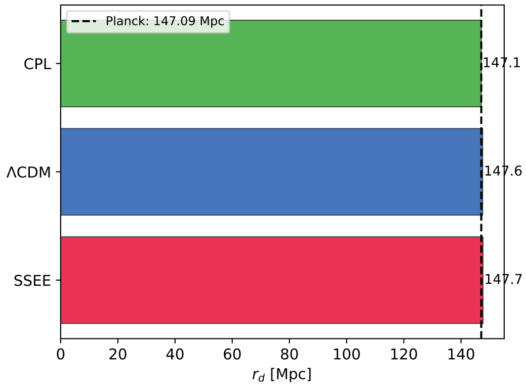
Sound horizon r_d (MAP) — SSEE matches \Lambda\text{CDM}
