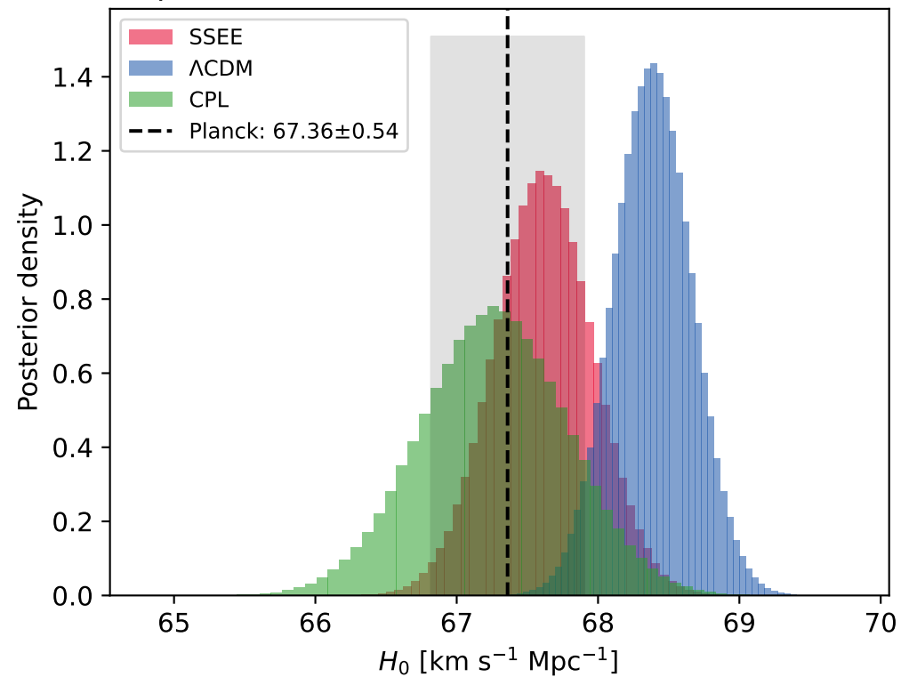
H_0 posteriors — SSEE 67.62 \pm 0.35 ( 0.40\sigma Planck)
