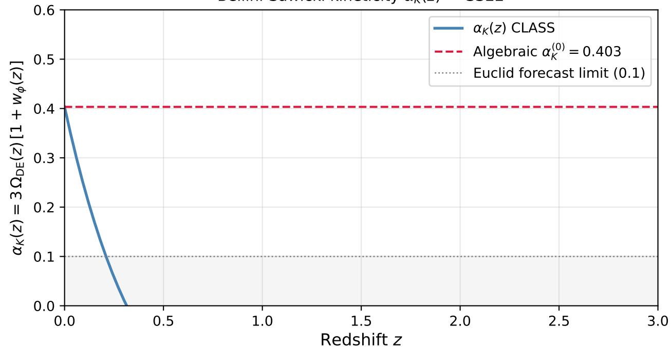
Bellini-Sawicki kinematicity \alpha_K(z) — SSEE
