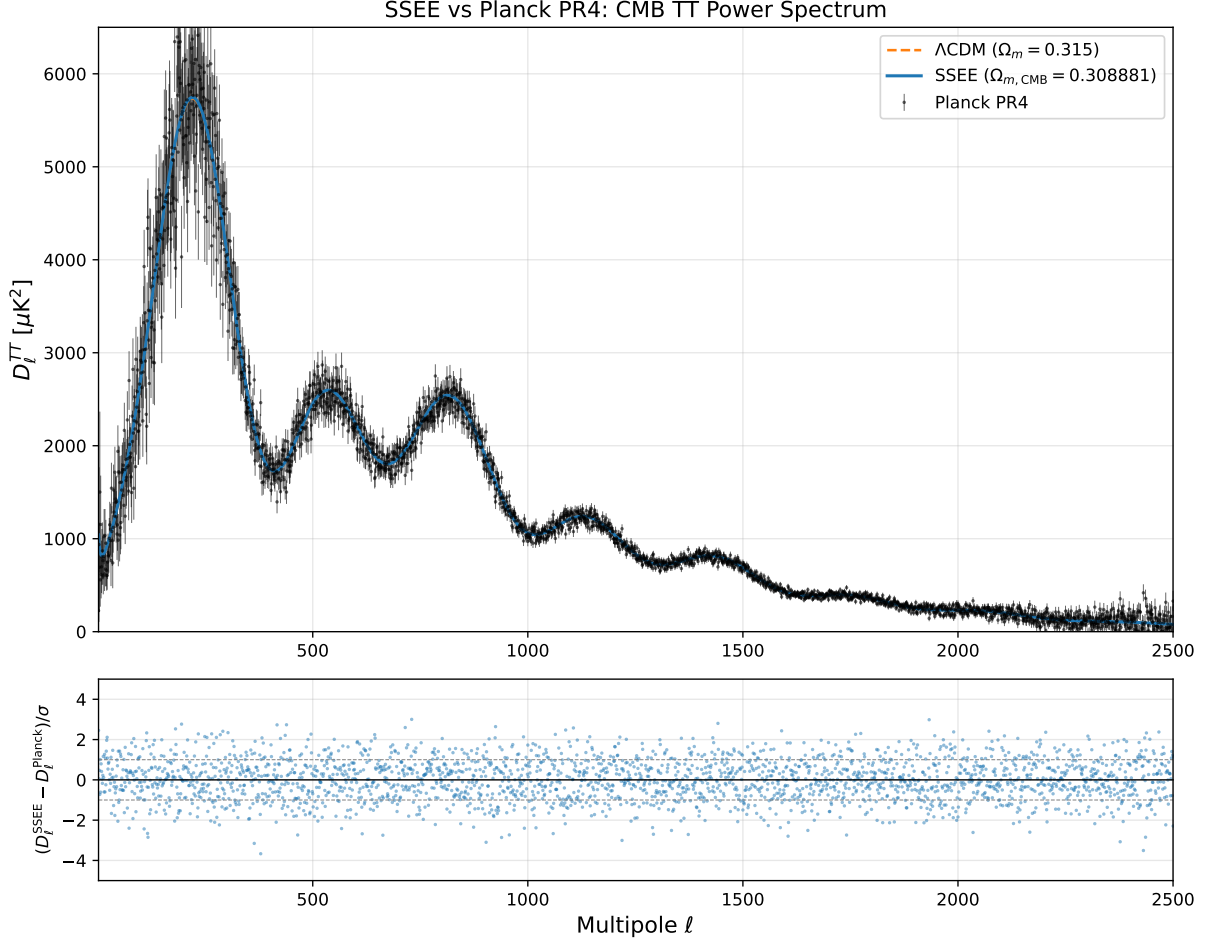
Figure 1: CMB TT power spectrum D_\ell^{TT} [ \mu\text{K}^2 ] vs. multipole \ell . Blue: SSEE ( \Omega_{m,\text{CMB}} = \omega_m/h^2 = 0.309 , w_0 = -0.839950 , w_a = -0.669975 ). Orange dashed: \Lambda CDM Planck 2018 best-fit. Black points: Planck PR4 TT data with \pm 1\sigma error bars. Lower panel: residuals (D_\ell^{\text{SSEE}} - D_\ell^{\text{Planck}})/\sigma .
