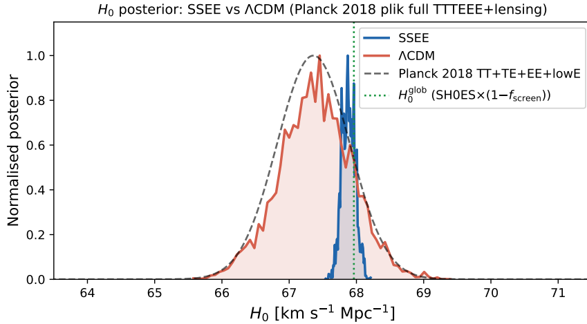
Figure 6: H_0 marginalised posterior for SSEE (blue) and \Lambda CDM (red) from the B1 full plik MCMC. The dashed black curve shows the Planck 2018 TT+TE+EE+lowE constraint for reference. The dotted green line marks the SSEE global rate H_0^{\text{glob}} = 67.96214 \text{ km s}^{-1} \text{ Mpc}^{-1} . In the validation chain (where H_0 is floated) SSEE places H_0 at 67.88 \pm 0.10 , 0.81\sigma from H_0^{\text{glob}} ; the model itself carries only two free parameters \{A_s, \tau\} , with H_0 derived. The narrow constraint ( \pm 0.10 \text{ km s}^{-1} \text{ Mpc}^{-1} ) reflects the removal of the H_0 - \Omega_m degeneracy by algebraically fixing \Omega_{m,\text{CMB}} = 0.3089 .
