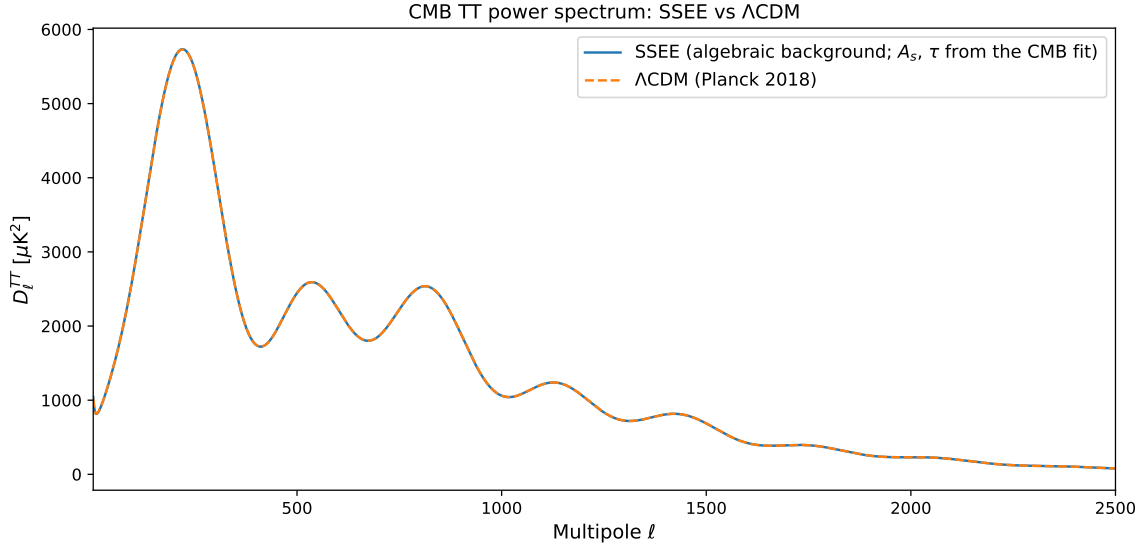
Figure 1: SSEECMB TT power spectrum ( k = 2 : A_s and \tau from the model’s own CMB fit; \omega_b, \omega_c, n_s, w_0, w_a, H_0 and \sum m_\nu algebraic from \varphi, \pi ), overlaid on the Planck 2018 \Lambda CDM spectrum computed in the same way. SSEE acoustic peak positions: \ell_1 = 220, \ell_2 = 536, \ell_3 = 813 ; \Lambda CDM: 220, 536, 813. The background is not fitted to CMB data; the peak positions follow from it.
