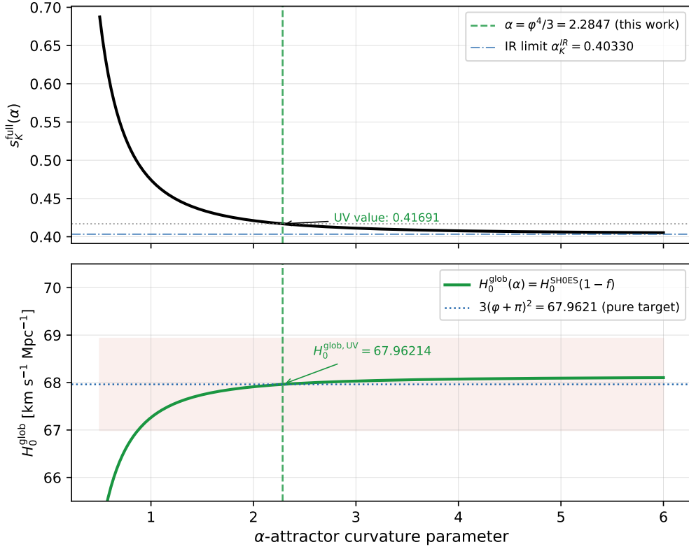
Figure 2: Top : Full screening rate s_K^{\text{full}}(\alpha) as the inflationary curvature \alpha varies. At \alpha = \varphi^4/3 = 2.284701 (green dashed), s_K^{\text{full}} = 0.41691 (green dot); the IR limit 0.40330 is shown dash-dotted blue. Bottom : Global background rate H_0^{\text{glob}}(\alpha) returned by the cascade Eq. (21) from the measured H_0^{\text{SH0ES}} = 73.04 \pm 1.04 km/s/Mpc (solid green); the dotted blue line is the dimensionless target 3(\varphi + \pi)^2 = 67.96214 and the shaded band is the propagated SH0ES uncertainty \pm 0.968 km/s/Mpc. If LiteBIRD measures r_{\text{obs}} , one reads off \alpha_{\text{obs}} = r_{\text{obs}}^2/12 and the x -axis gives the falsifiable output. At \alpha = \varphi^4/3 the cascade returns 67.96214 km/s/Mpc, i.e. 4.2 \times 10^{-6} from the target. Note that the band is far wider than that residual: the agreement is not a measurement of \alpha .
