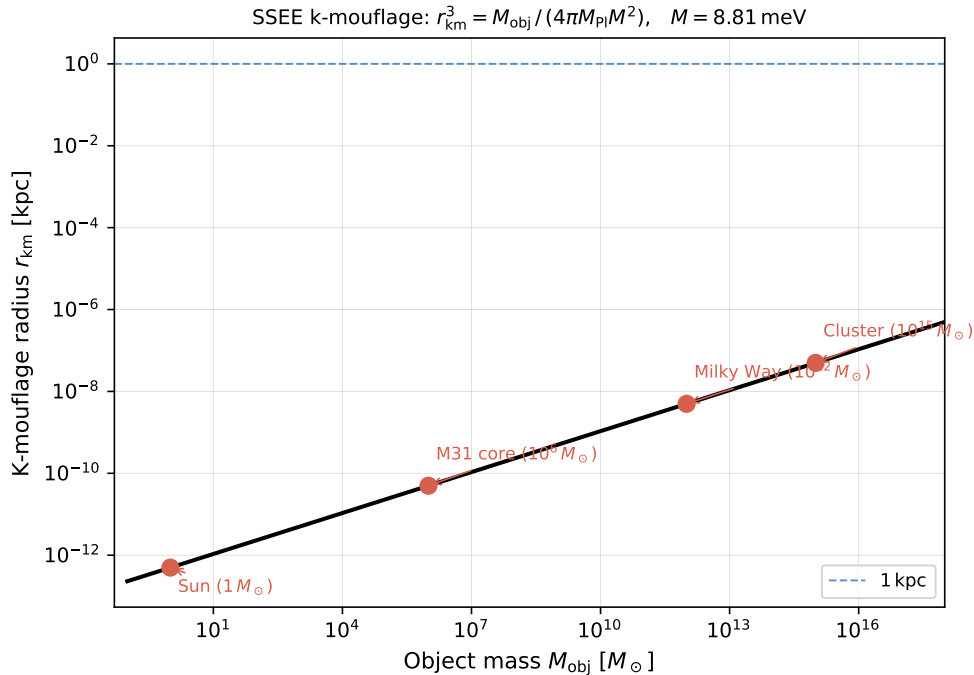
Figure 2: K-mouflage screening radius r_{\text{km}} = [M_{\text{obj}} / (4\pi M_{\text{Pl}} M^2)]^{1/3} as a function of object mass (in M_{\odot} ) at the UV completion scale M = 8.81 meV (Almeida Vallejo, 2026d; Brax & Valageas, 2014). For all representative objects, r_{\text{km}} lies far below the galactic scale, so DM fifth-force dynamics are active at cosmological radii while baryons remain decoupled through selective coupling (Section 6.3).
