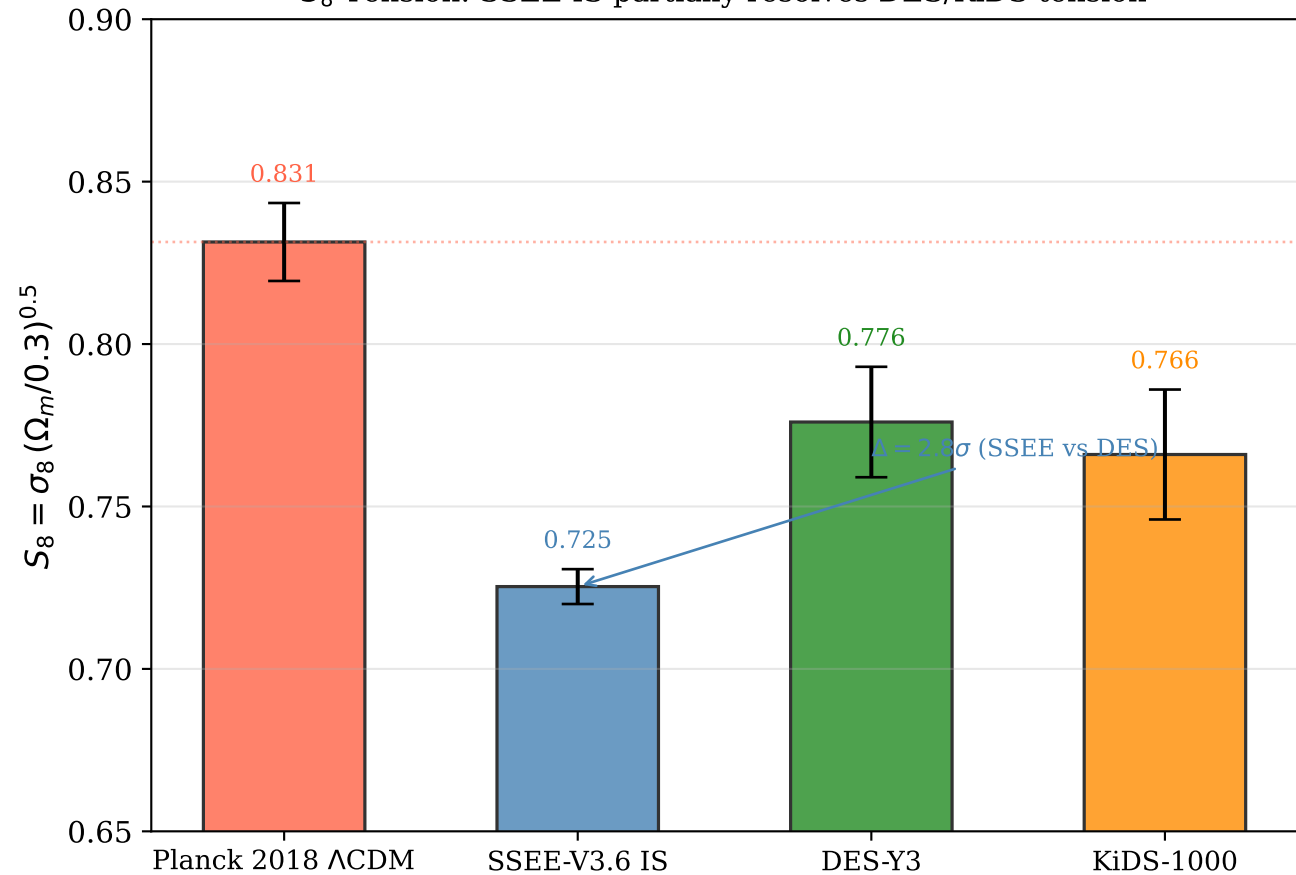
S_8 Tension: SSEE IS partially resolves DES/KiDS tension
