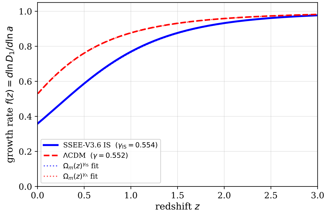
Growth Rate vs Redshift (SSEE IS vs \Lambda CDM)
