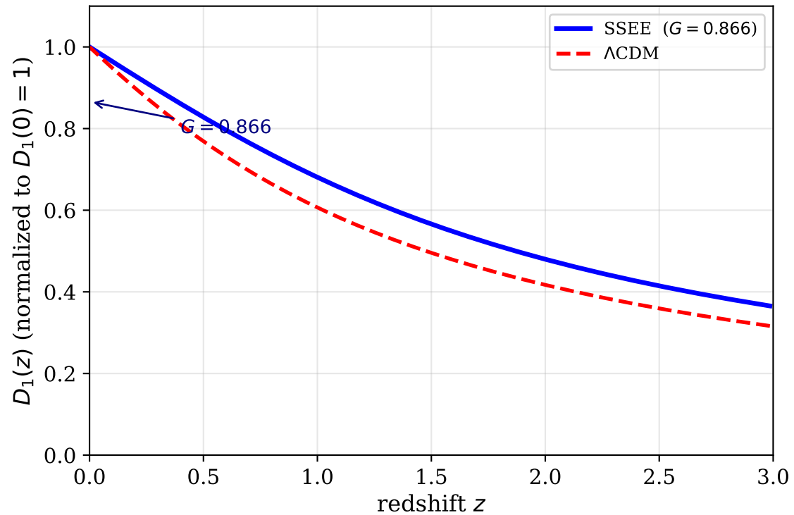
Growth Factor (normalized)
