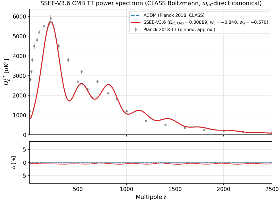
Figure 1: CMB TT power spectrum from CLASS. Blue dashed : \Lambda CDM Planck 2018. Red solid : SSEE with the full \omega_m -direct canonical matter density \Omega_{m,CMB} = 0.30889 ( w_0 = -0.840 , w_a = -0.670 ) — peaks at \ell = 221, 537, 814 , agreeing with \Lambda CDM to within \Delta\ell \leq 1 (RMS = 0.14%). Grey points: Planck 2018 binned TT (approximate). The SSEE dynamical-only run ( \Omega_{m,CMB} = 0.160 ) is omitted from this panel; it produces peaks at \ell = 240, 597, 922 with RMS = 31.5% relative to \Lambda CDM, confirming that the full matter density (not the dynamical \Omega_{m,dyn} = 0.160 ) is needed to reproduce the acoustic scale.
