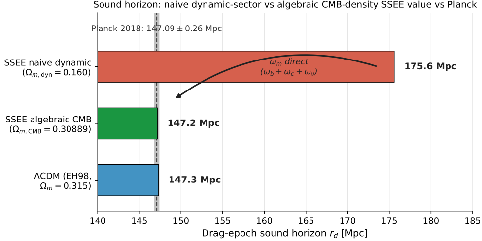
Figure 7: The physical sound horizon. Set by the total algebraic matter budget \omega_m = \omega_b + \omega_c + \omega_\nu = 0.14267 ( \Omega_m = \omega_m/h^2 = 0.30889 , \omega_m -direct, no matter factor), the SSEE drag scale is r_d = 147.17 \text{ Mpc} (CAMB; log p3_rd_reframe_omega_m ), consistent with the Planck-inferred 147.09 \pm 0.26 \text{ Mpc} (grey band, 0.32\sigma ) and the \Lambda\text{CDM} Eisenstein–Hu value (147.3 Mpc); the BAO-distance run gives 148.2 Mpc, matching \Lambda\text{CDM} to 0.2%. The 175.6 Mpc value that appears if the cold sector 1 + w_0 = 0.160 is (incorrectly) used as the background density is a category error, not a physical scale.
