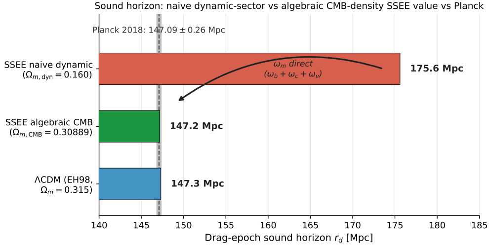
Figure 2: The physical sound horizon. Set by the full algebraic \omega_m (green, 147.17 Mpc at \Omega_m^{\text{cosm}} = 0.30889 , \omega_m -direct), in agreement with Planck 2018 ( 147.09 \pm 0.26 Mpc, grey band) and the \Lambda CDM Eisenstein–Hu value (blue, 147.3 Mpc); the BAO-distance run gives 148.2 Mpc. This is the visual counterpart of the Boltzmann test above: the full matter density that restores the acoustic peaks also restores the BAO standard ruler. The 175.6 Mpc scale (red) is the category error of using the cold sector \Omega_m^{\text{dyn}} = 0.160 as the background density.
