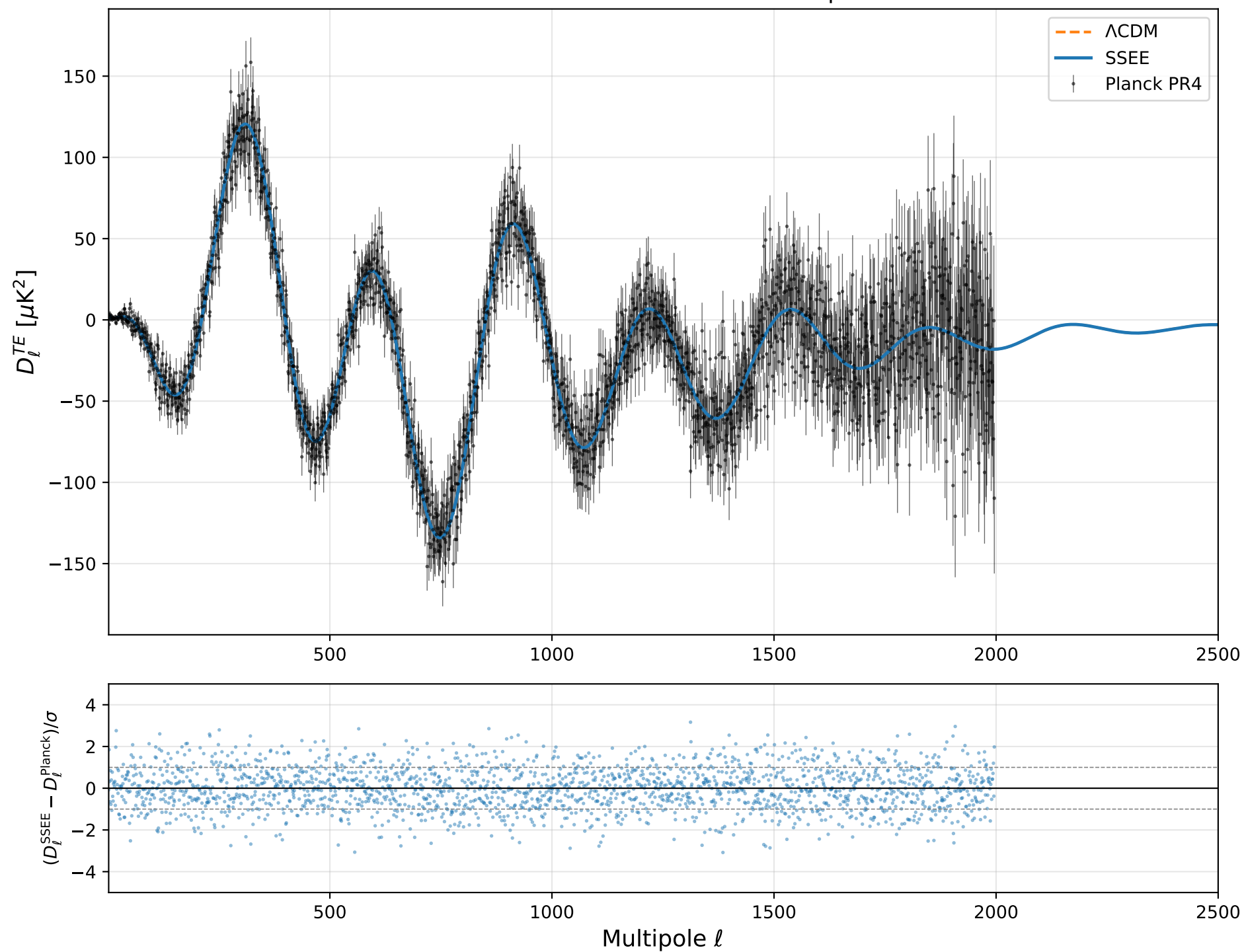
SSEE vs Planck PR4: CMB TE Power Spectrum
