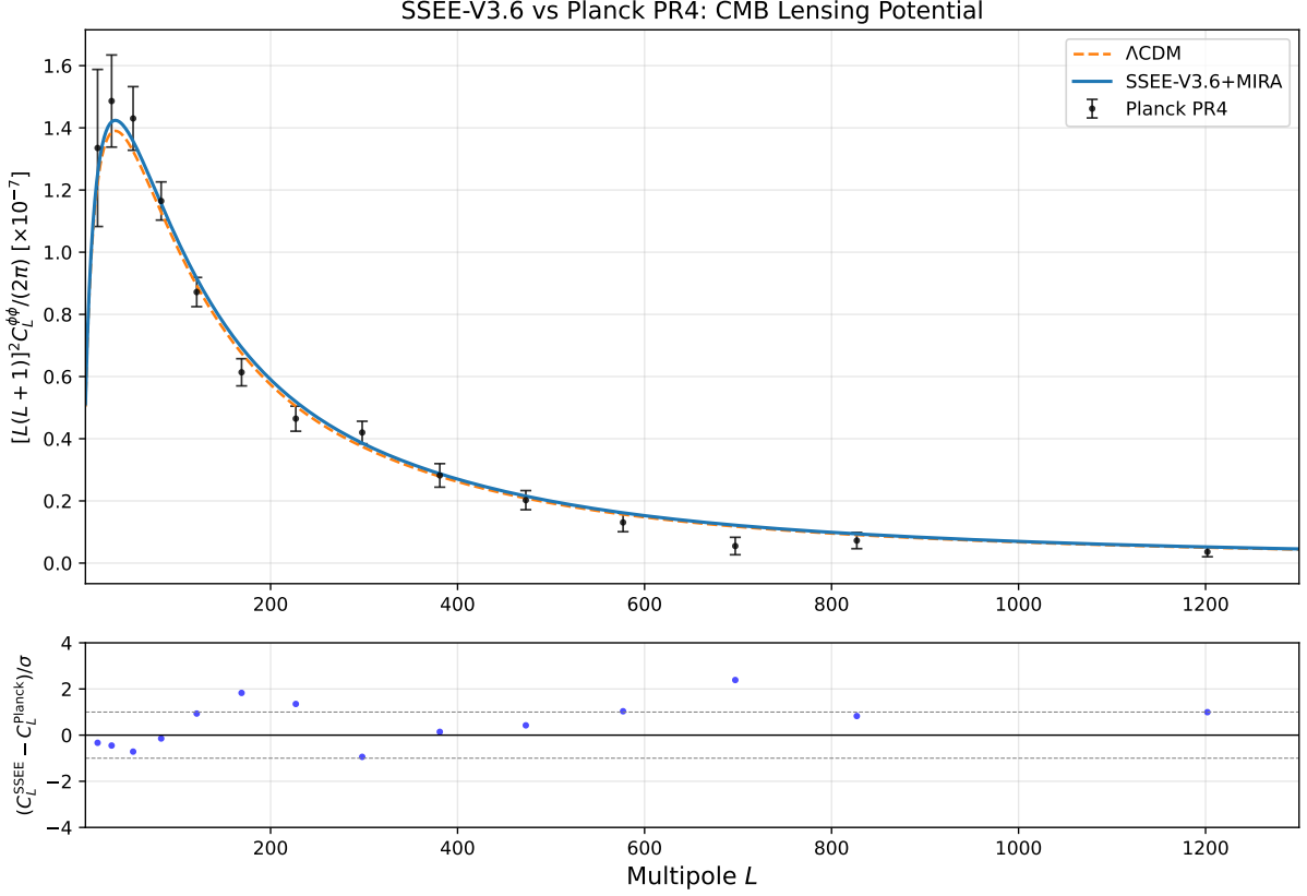
Figure 5: CMB lensing potential power spectrum [L(L + 1)]^2 C_L^{\phi\phi} / (2\pi) . Blue: SSEE+MIRA. Orange dashed: \Lambda CDM. Black points: Planck PR4 lensing (9 MV band-powers). Lower panel: residuals normalised by \sigma_L . SSEE achieves \chi_r^2 = 0.866 over the 9 bandpowers (§5.4; \Lambda CDM: 0.757), both indicating a good fit ( \chi_r^2 < 1 ).
