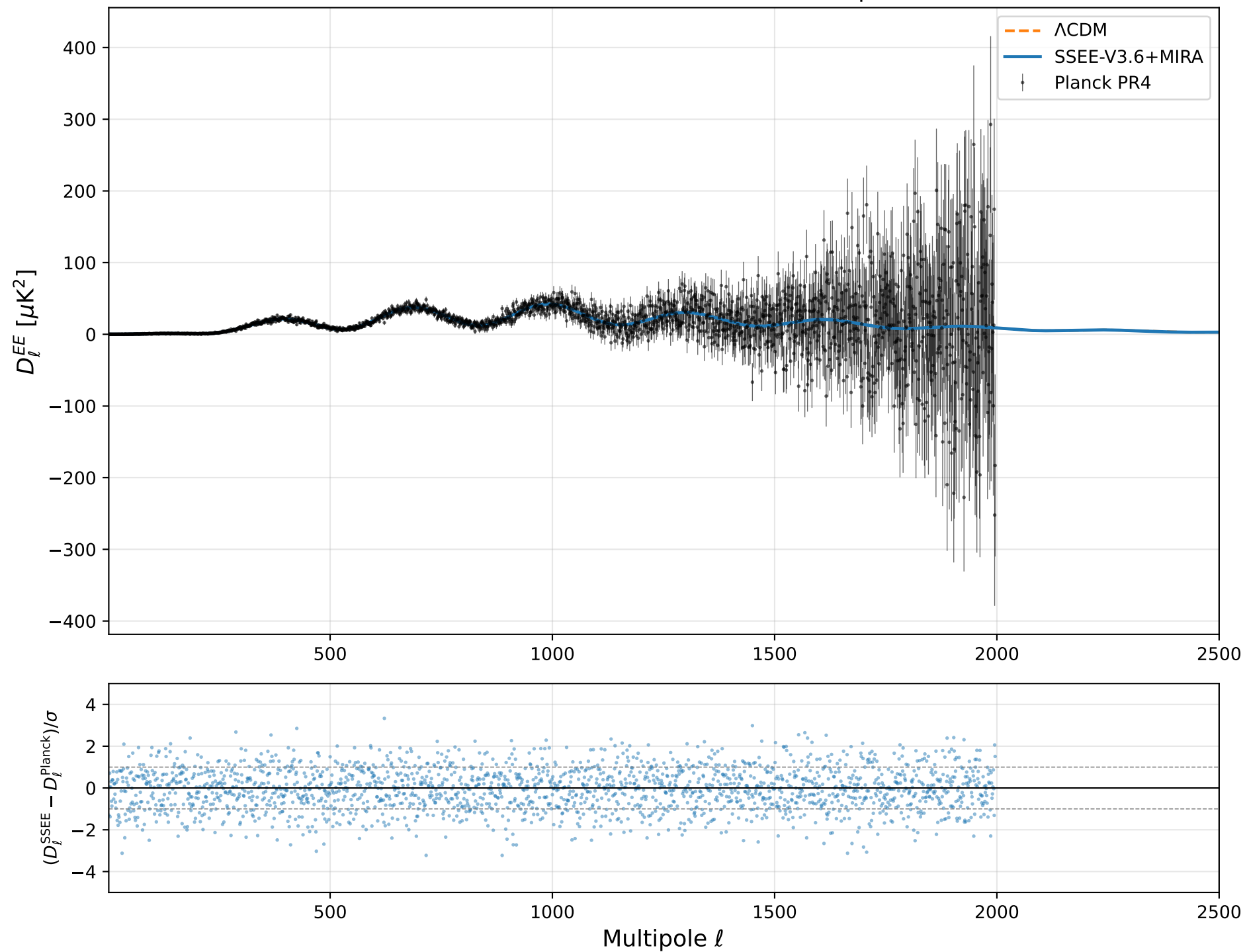
SSEE-V3.6 vs Planck PR4: CMB EE Power Spectrum
