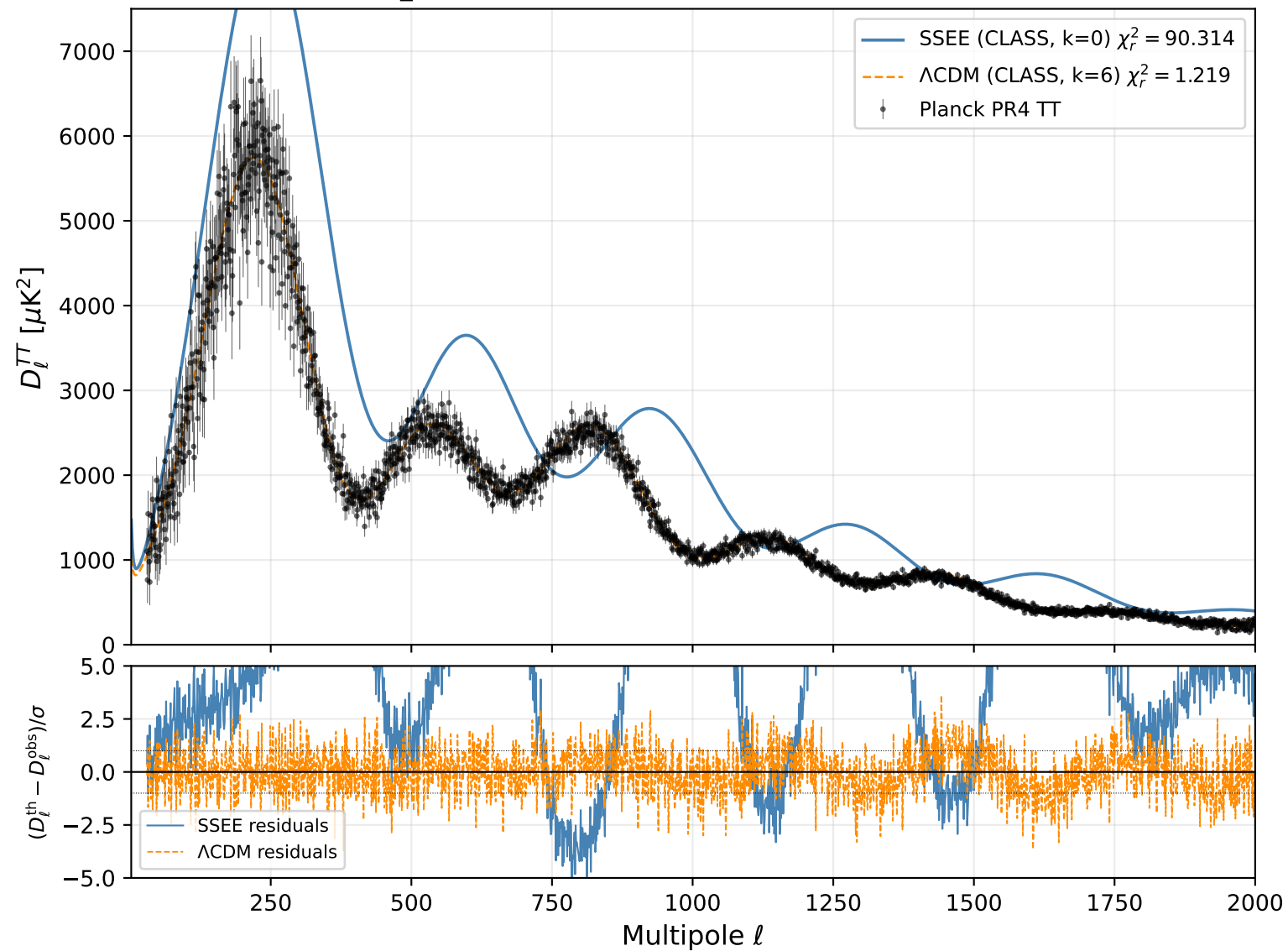
hi_class cross-check — SSEE-V3.6 vs Planck PR4 TT
