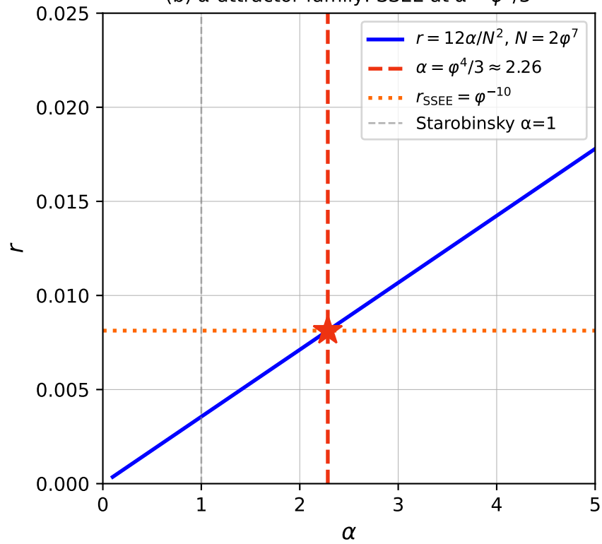
(b) \alpha -attractor family: SSEE at \alpha = \varphi^4/3
