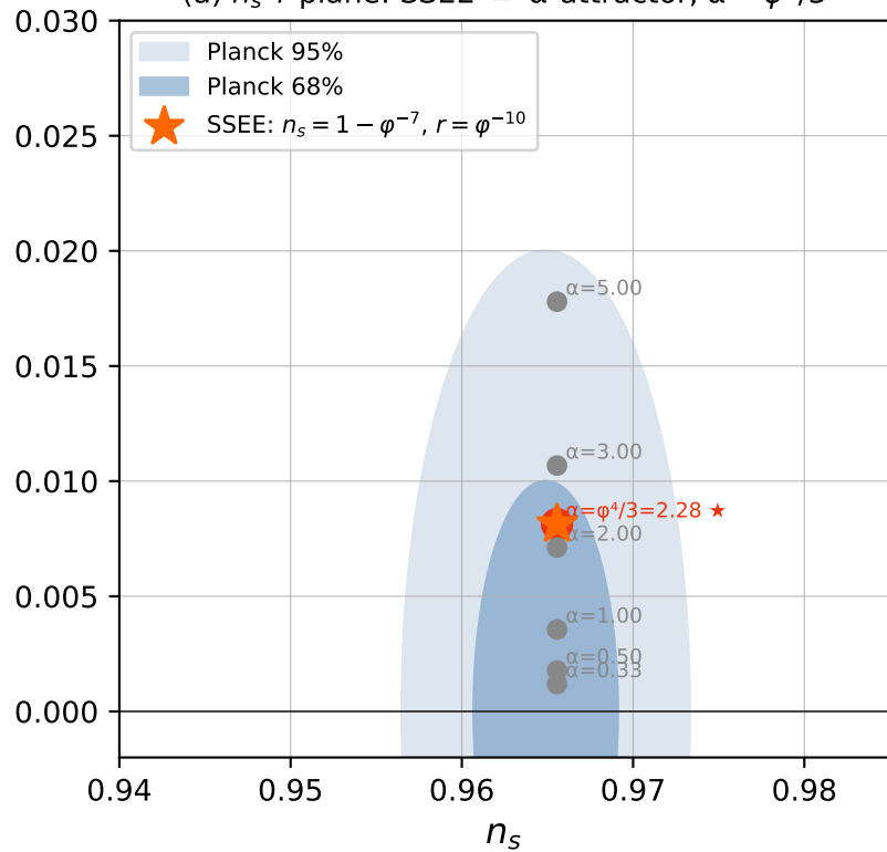
(a) n_s - r plane: SSEE \equiv \alpha -attractor, \alpha = \varphi^4/3
