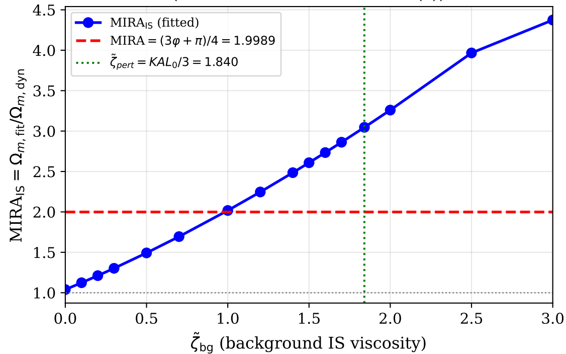
MIRA from Background IS (\Lambda\text{CDM fit to IS-modified } H(z))
