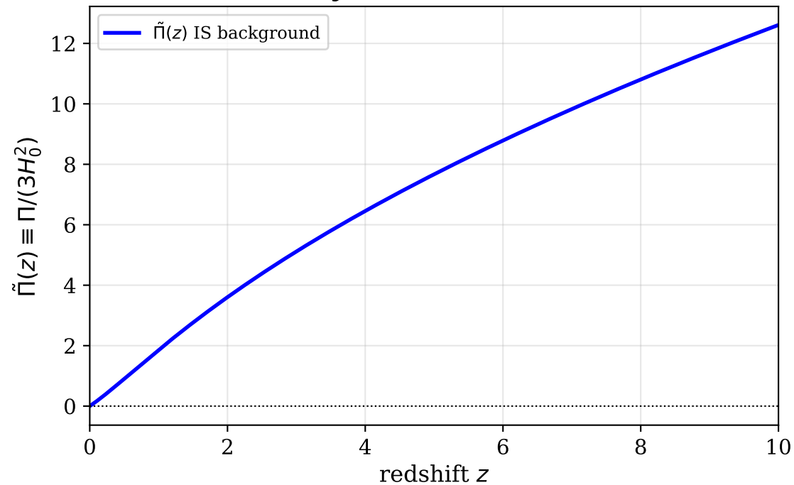
IS Bulk Pressure Background (\tilde{\zeta}_{\text{bg}} = KAL_0/3 = 1.840)
