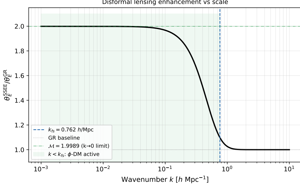
Figure 1: Disformal lensing enhancement \theta_E^{\text{SSEE}}/\theta_E^{\text{GR}} as a function of wavenumber k (h/Mpc). For k < k_{\text{fs}} = 0.762 \text{ h/Mpc} (blue dashed), the \phi -DM sector is active and the ratio approaches the algebraic limit \sqrt{\beta_c} = \sqrt{\mathcal{A}} \approx 1.9995 (dashed-dotted green), equivalent to \mathcal{M} = 1.999 . For k > k_{\text{fs}} the \phi -DM free-streams, the scalar gradient decouples, and lensing recovers the GR baseline (dotted). This is the pedagogical limit (a) (disformal scalar-force enhancement); the canonical limit (b) of the actual SSEE model recovers GR-with-DM lensing on all scales (Sec. 6.4).
