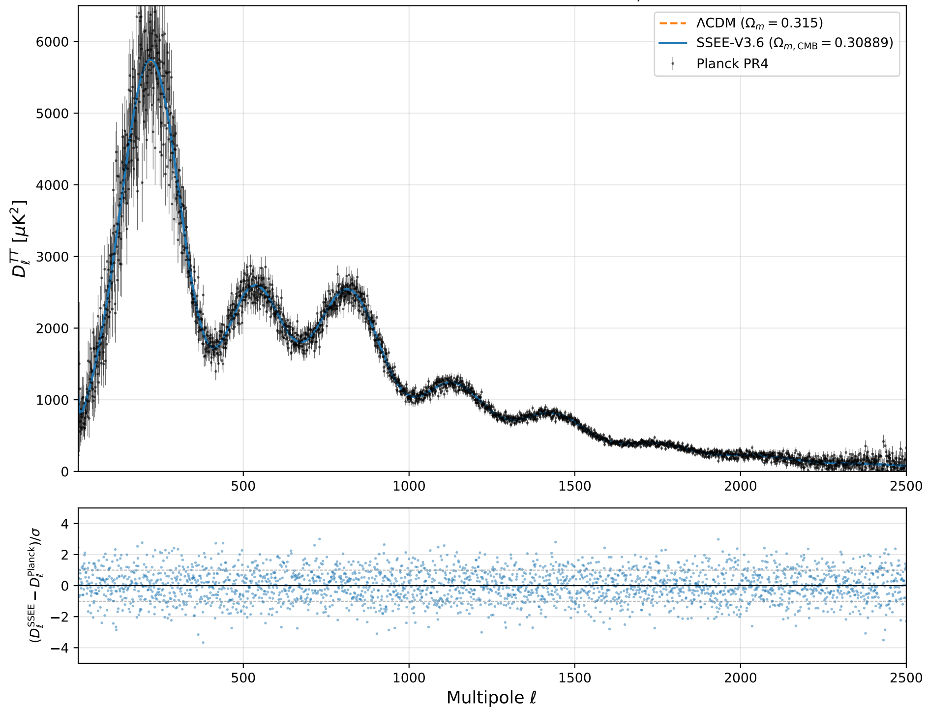
SSEE-V3.6 vs Planck PR4: CMB TT Power Spectrum
