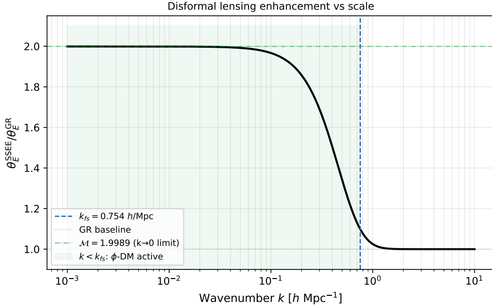
Figure 1: Disformal lensing enhancement \theta_E^{\text{SSEE}}/\theta_E^{\text{GR}} as a function of wavenumber k (h/Mpc). For k < k_{\text{fs}} = 0.754 \text{ h/Mpc} (blue dashed), the \phi -DM sector is active and the ratio approaches the algebraic limit \sqrt{\beta_c} = \sqrt{\mathcal{A}} \approx 1.9995 (dashed-dotted green), equivalent to \mathcal{M} = 1.999 . For k > k_{\text{fs}} the \phi -DM free-streams, the scalar gradient decouples, and lensing recovers the GR baseline (dotted). This is the pedagogical limit (a) (disformal scalar-force enhancement); the canonical limit (b) of the actual SSEE model recovers GR-with-DM lensing on all scales (Sec. ??).
