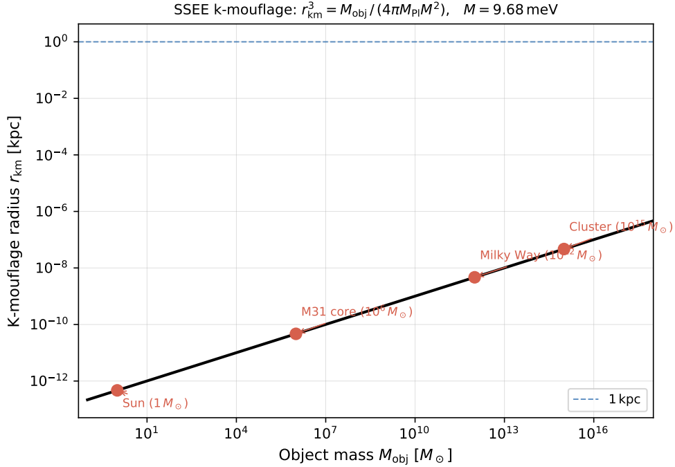
Figure 2: K-mouflage screening radius r_{\text{km}} = [M_{\text{obj}}/(4\pi M_{\text{Pl}} M^2)]^{1/3} as a function of object mass (in M_\odot ) at the UV completion scale M = 9.68 \text{ meV} (?). For all representative objects, r_{\text{km}} lies far below the galactic scale, so DM fifth-force dynamics are active at cosmological radii while baryons remain decoupled through selective coupling (Section ??).
