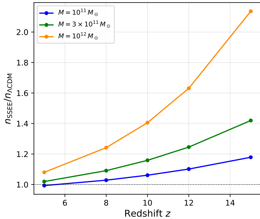
Enhancement vs redshift
