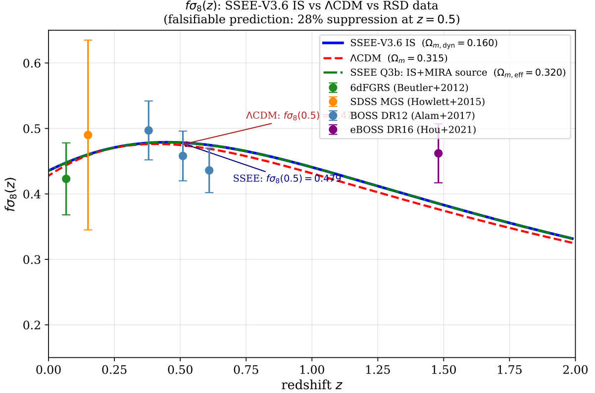
Figure 3: f\sigma_8(z) for SSEE-V3.6 IS (solid blue) and \Lambda CDM (dashed red) versus RSD measurements from 6dFGRS [?], SDSS MGS [?], BOSS DR12 [?], and eBOSS DR16 [?]. The SSEE prediction ( \Omega_{m,\text{cosm}} = 0.320 in growth equation) is essentially identical to \Lambda CDM at z < 1 , with a mean tension of 0.74\sigma across six data points (vs. 0.73\sigma for \Lambda CDM).
