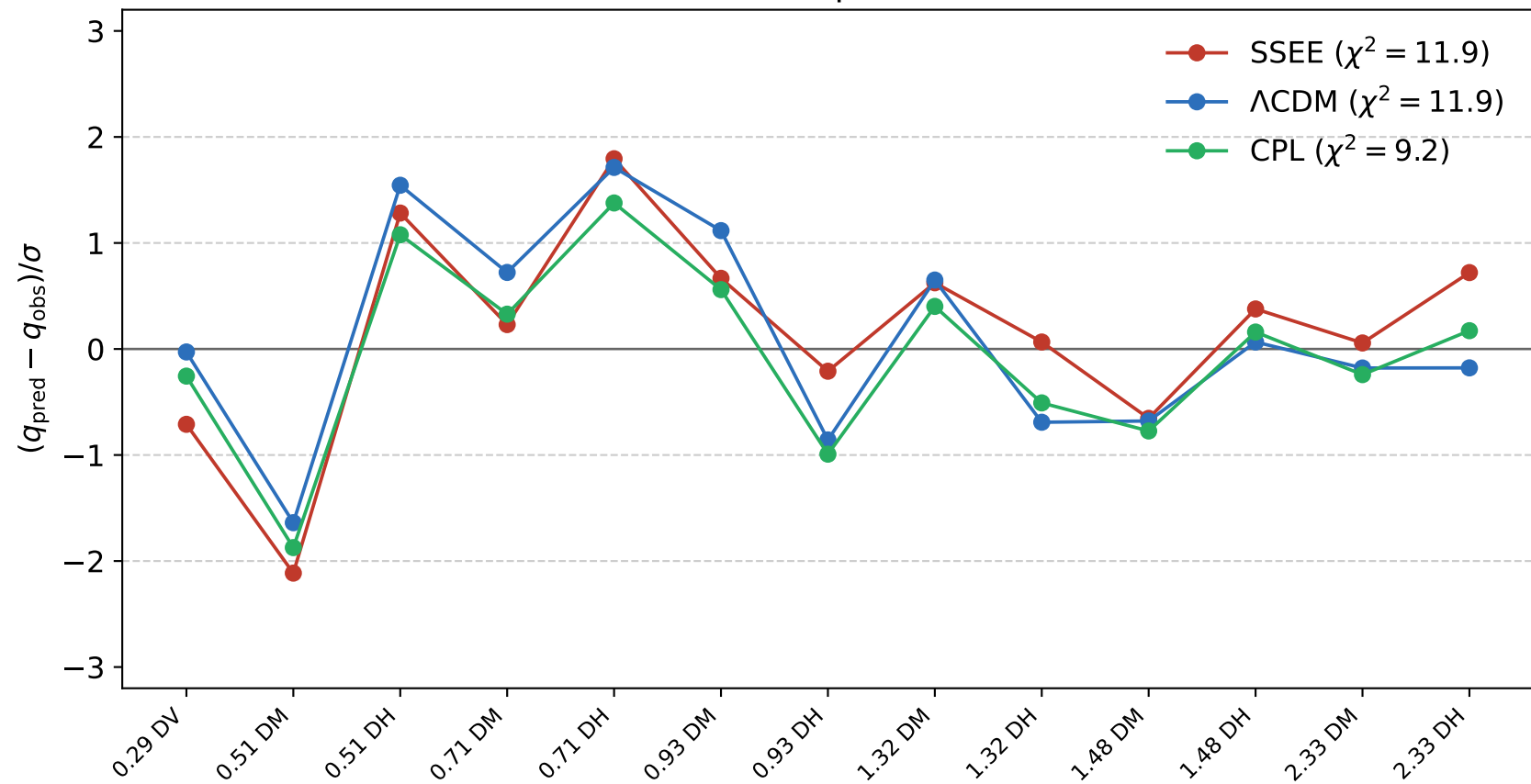
DESI DR2 BAO residuals (13 points, 2503.14738 Table 4)
