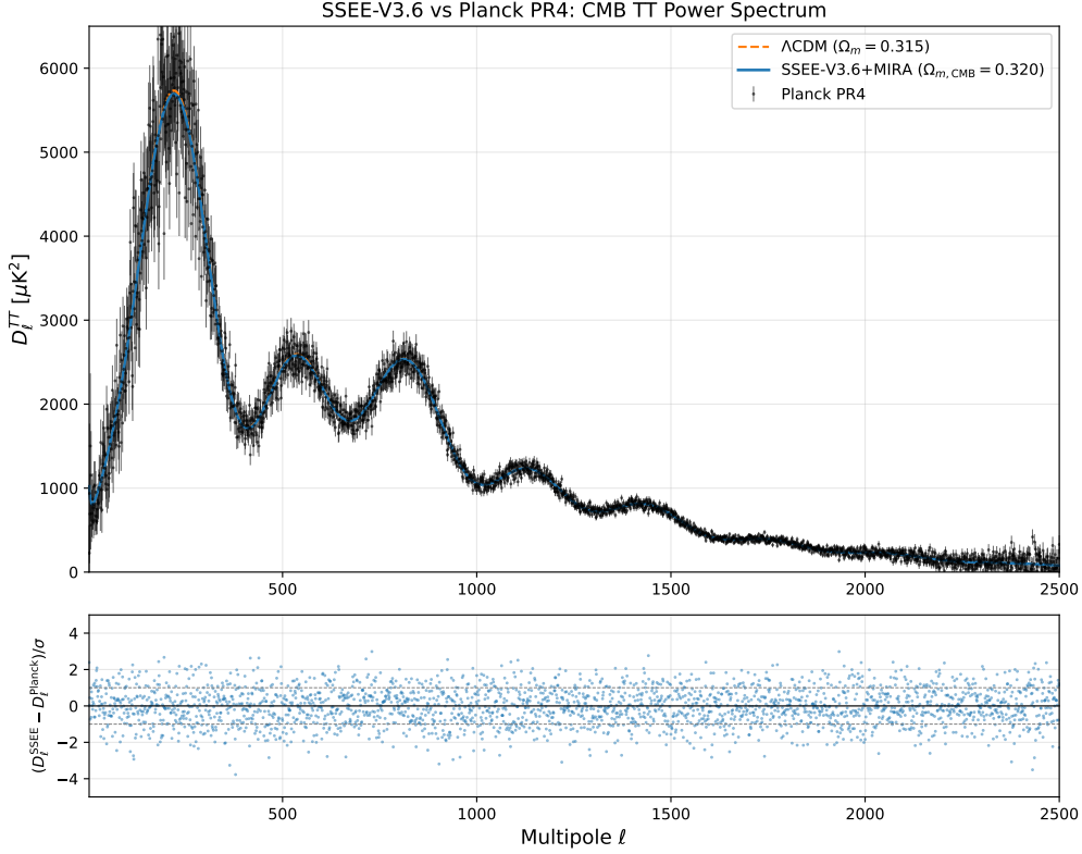
Figure 3: CMB temperature angular power spectrum computed with CLASS for the SSEE background and EFT functions (Eq. ??), compared against Planck PR4. With the dark-energy sector fixed by \varphi and \pi , SSEE reproduces the acoustic peaks at \ell = 220, 535, 810 at a quality indistinguishable from \Lambda CDM (Table ??). The two- \Omega_m structure is essential: replacing \Omega_m^{\text{cosm}} = 0.320 with the bare \Omega_m^{\text{dyn}} = 0.160 shifts every peak by \sim 10\% .
