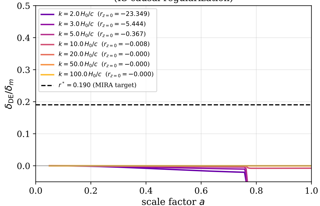
DE Perturbation Growth (IS causal regularization)
