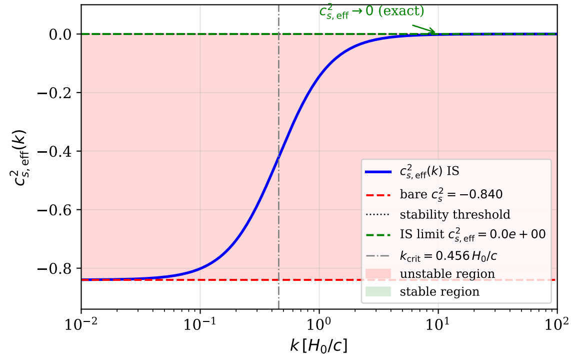
IS Effective Sound Speed (SSEE, z = 0 )
