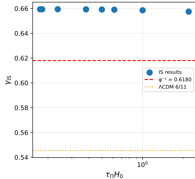
Growth index scan
