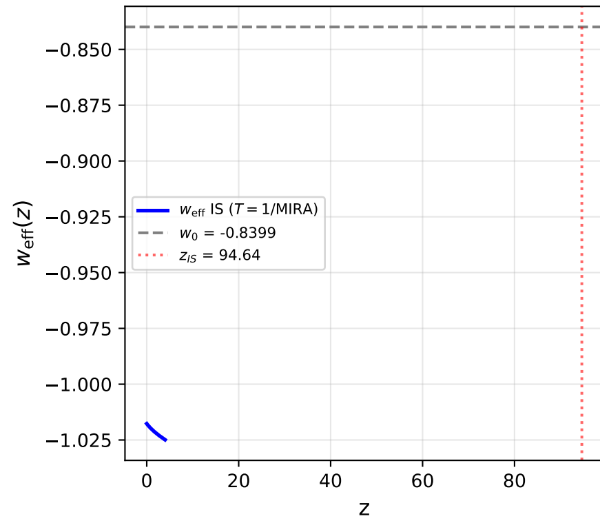
IS effective EOS
