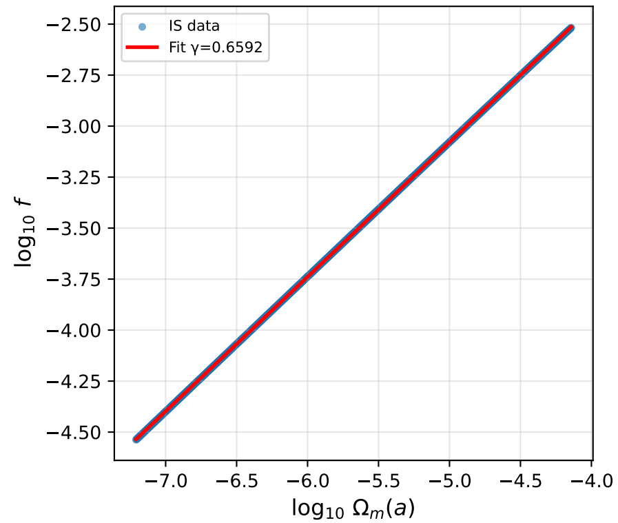
Growth rate f \approx \Omega_m^\gamma
