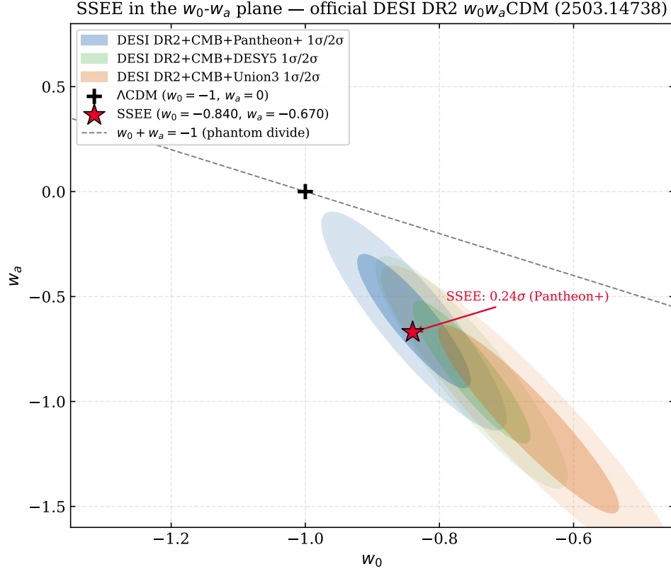
FIG. 1. The SSEE prediction in the w_0 - w_a plane. The single point (w_0, w_a) = (-T_r/M_v, -P_{sc}/K_v) = (-0.840, -0.670) is fixed entirely by \varphi and \pi , with no dark-energy parameters adjusted to the data. The shaded contours are the official DESI DR2 w_0w_a CDM posteriors (Pantheon+, DESY5, Union3). The SSEE point falls inside the Pantheon+ 1\sigma region; the joint Mahalanobis distance is \chi^2_{2D} = 0.42 , an equivalent 0.24\sigma agreement (Eq. 2), and within 1.5 – 1.8\sigma of the other compilations.
