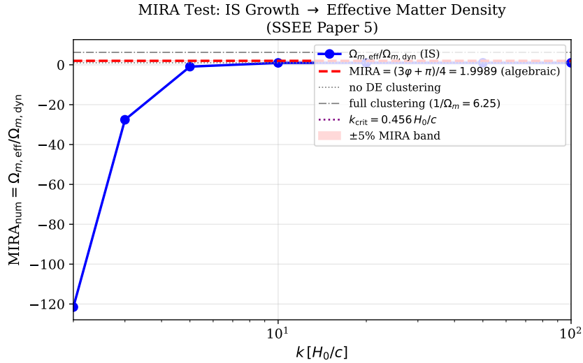
Figure 2: MIRA num ( k ) (blue points with error bars) versus k/(H_0/c) . The algebraic target MIRA = (3\varphi + \pi)/4 \simeq 1.999 (red dashed) is not approached: IS suppression drives MIRA num \rightarrow 1 for k \gg H_0/c . The grey region marks full DE clustering ( 1/\Omega_{m,\text{dyn}} \simeq 6.25 ), ruled out by all current observations. The required perturbation amplitude r^* = 0.190 (Eq. 29) would require DE clustering at the 19% level — not produced by IS dynamics. The conclusion is that MIRA is not reproduced by IS dynamics: linear perturbations yield MIRA num \approx 1 , not 1.9989; and the background IS Friedmann integration gives a ratio \approx 3.04 , also failing to recover 1.9989. The MIRA factor remains a pure algebraic postulate; see Section 7.1.
