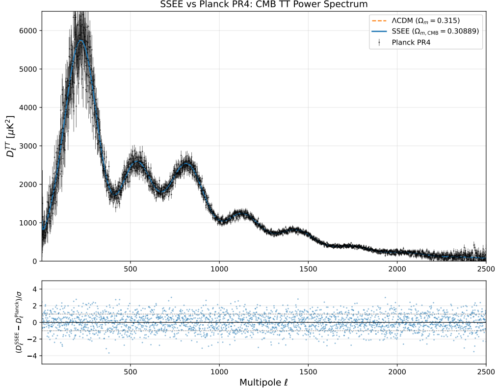
FIG. 4. CMB temperature angular power spectrum computed with CLASS for the SSEE background and EFT functions (Eq. 9), compared against Planck PR4. With the dark-energy sector fixed by \varphi and \pi , SSEE reproduces the acoustic peaks at \ell = 220, 535, 810 at a quality indistinguishable from \Lambda CDM (Table IV). The two- \Omega_m structure is essential: replacing \Omega_m^{\text{cosm}} = 0.30889 with the bare \Omega_m^{\text{dyn}} = 0.160 shifts every peak by \sim 10\% .
