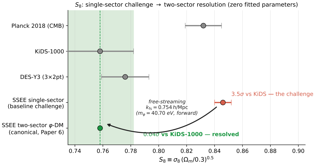
FIG. 5. S_8 : the single-sector challenge and the two-sector resolution. The single-sector ceiling (red, S_8 = 0.846 \pm 0.006 ) carries the 3.5\sigma tension with KiDS-1000 reported in Eq. (13); the two-sector \varphi -DM extension (green, S_8 = 0.758 ) lands 0.04\sigma from KiDS-1000 (green band), with the free-streaming scale fixed by the forward-predicted mass m_\varphi = 40.70 \text{ eV} — no parameter fitted to lensing data. Grey points: Planck 2018, KiDS-1000 and DES-Y3 with 1\sigma errors.
