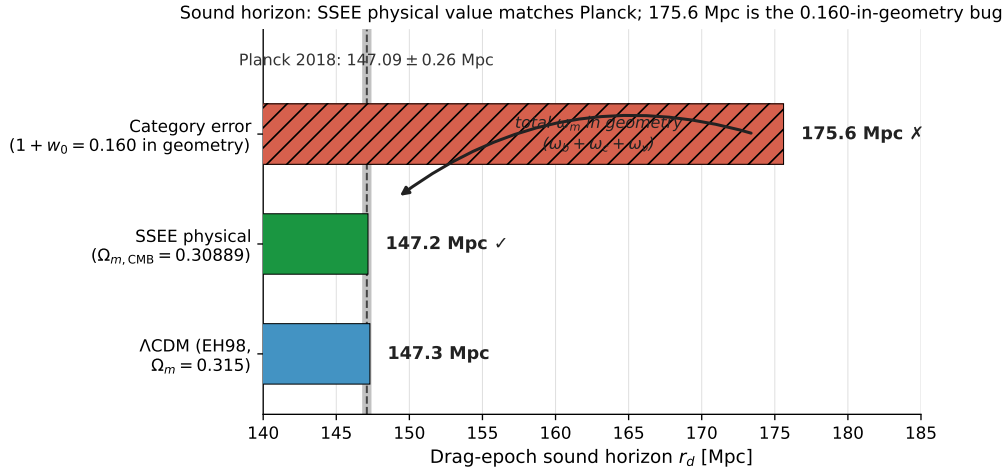
FIG. 2. The physical sound horizon. Set by the full algebraic \omega_m (green, 147.17 Mpc at \Omega_m^{\text{cosm}} = 0.30889 , \omega_m -direct), in agreement with Planck 2018 ( 147.09 \pm 0.26 Mpc, grey band) and the \Lambda CDM Eisenstein–Hu value (blue, 147.3 Mpc); the BAO-distance run gives 148.2 Mpc. This is the visual counterpart of the Boltzmann test above: the full matter density that restores the acoustic peaks also restores the BAO standard ruler. The 175.6 Mpc scale (red) is the category error of using the cold sector \Omega_m^{\text{dyn}} = 0.160 as the background density.
