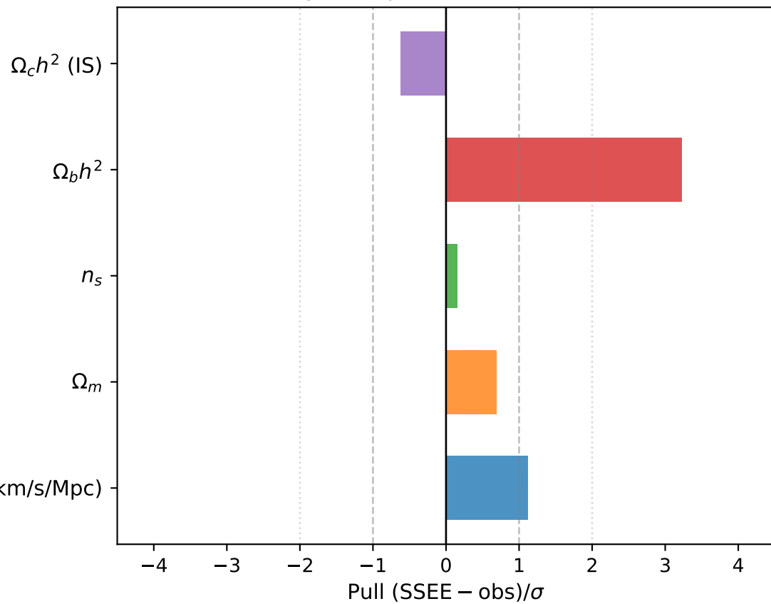
SSEE algebraic predictions vs Planck 2018
