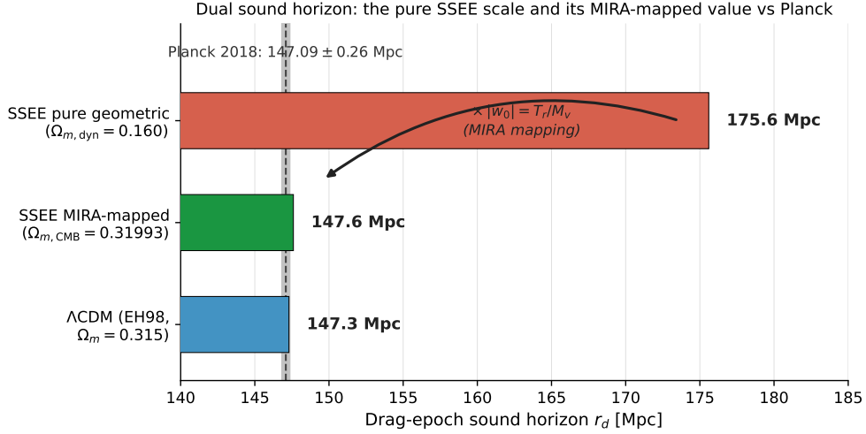
Figure 7: The dual sound horizon, visualised. The pure geometric SSEE drag scale is r_d = 175.6 \text{ Mpc} ( \Omega_{m,\text{dyn}} = 0.160 ); the MIRA mapping ( \times |w_0| = T_r/M_v ) carries it to r_d = 147.6 \text{ Mpc} ( \Omega_{m,\text{CMB}} = 0.31993 ), consistent with the Planck-inferred value 147.09 \pm 0.26 \text{ Mpc} (grey band) and the \Lambda\text{CDM} Eisenstein–Hu value (147.3 Mpc). The 175.6 Mpc scale shown in Fig. 6 is therefore the pre-mapping geometric quantity, not the model’s prediction for the observed BAO scale.
