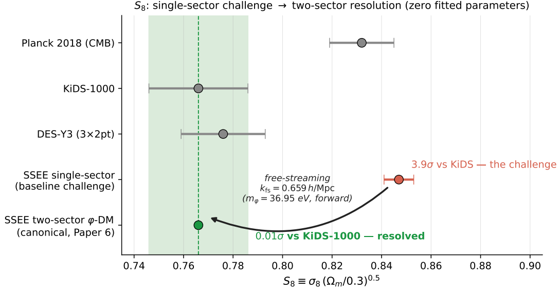
Figure 5: S_8 : the single-sector challenge and the two-sector resolution. The single-sector prediction (red, S_8 = 0.847 \pm 0.006 ) carries the 3.9\sigma tension with KiDS-1000 reported in Eq. (12); the two-sector \varphi -DM extension (green, S_8 = 0.766 ) lands 0.01\sigma from KiDS-1000 (green band), with the free-streaming scale fixed by the forward-predicted mass m_\varphi = 36.95 eV — no parameter fitted to lensing data. Grey points: Planck 2018, KiDS-1000 and DES-Y3 with 1\sigma errors.
