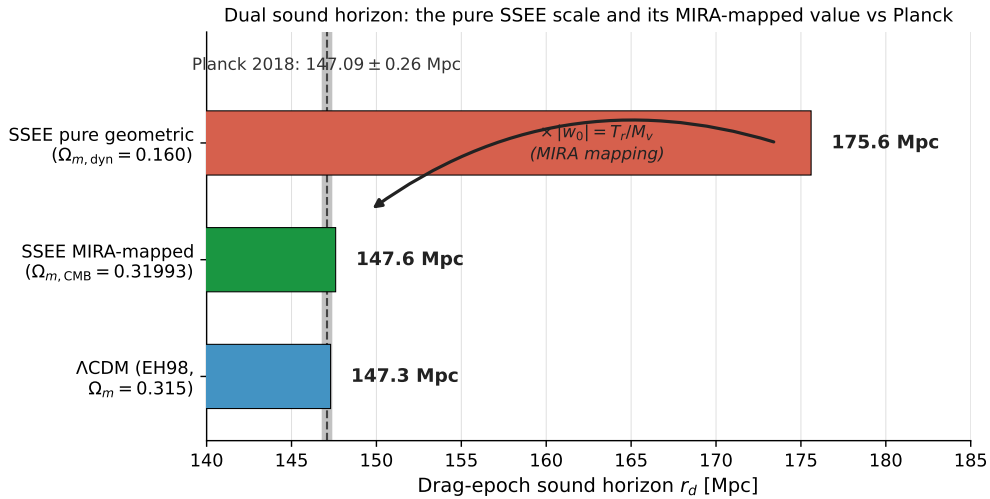
Figure 2: The dual sound horizon. The pure geometric SSEE drag scale (red, 175.6 Mpc) is carried by the MIRA mapping to 147.6 Mpc (green), in agreement with Planck 2018 ( 147.09 \pm 0.26 Mpc, grey band) and the \Lambda CDM Eisenstein–Hu value (blue, 147.3 Mpc). This is the visual counterpart of the Boltzmann test above: the same single algebraic constant that restores the acoustic peaks also restores the BAO standard ruler.
