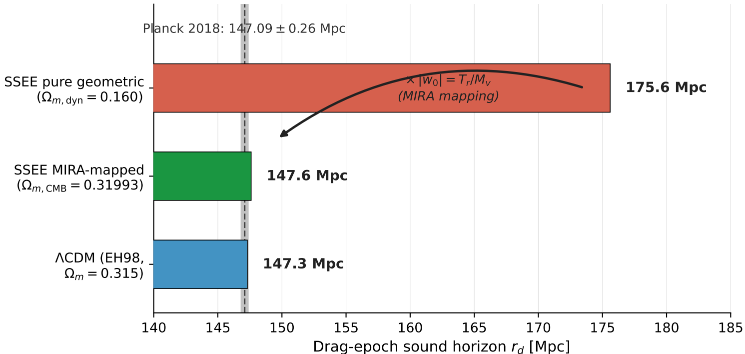
Dual sound horizon: the pure SSEE scale and its MIRA-mapped value vs Planck
