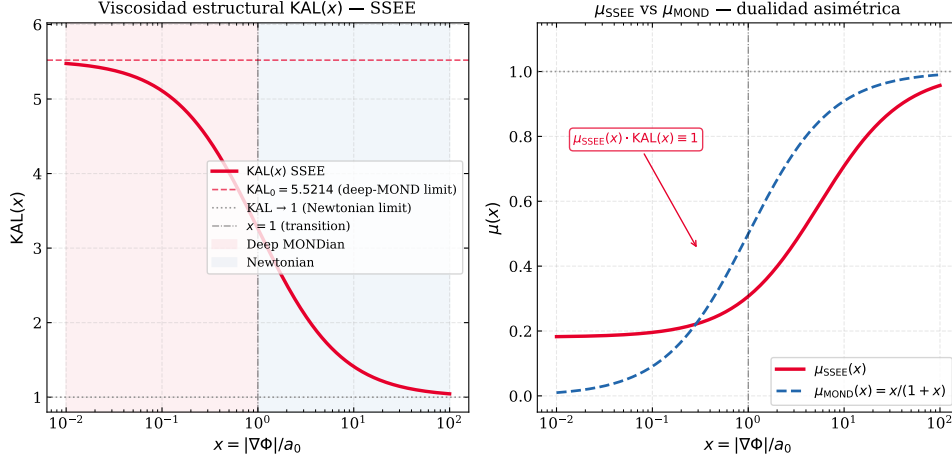
Figure 2: KAL(x) interpolation between the Newtonian limit ( x \gg 1 ) and the MONDian limit ( x \ll 1 ). The fixed point KAL_0 \approx 5.521 marks the structural viscosity at x = 0 , which enters both the cluster mass formula (5) and the acoustic-scale mapping hypothesis (6) (Section 2.4).
