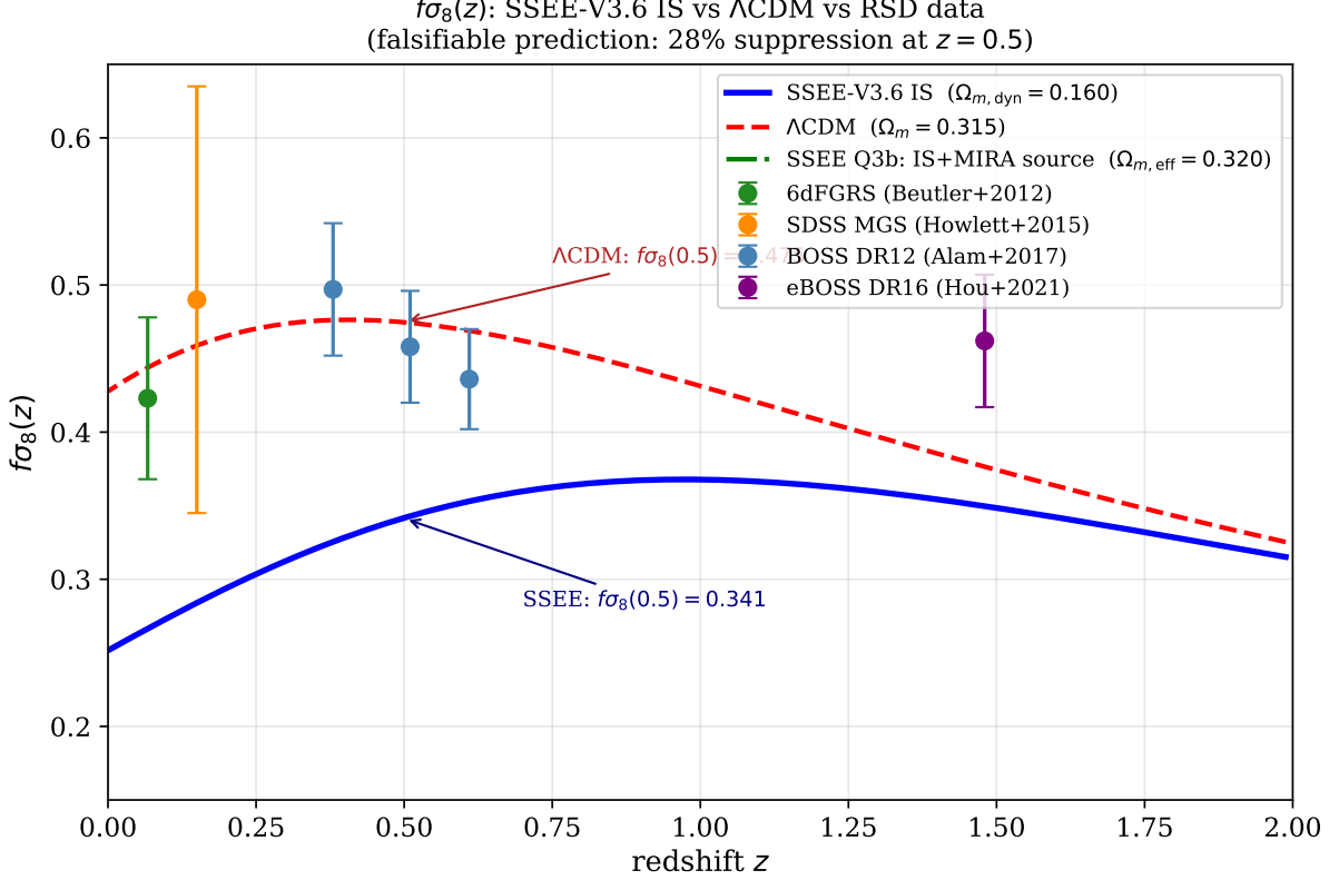
Figure 3: f\sigma_8(z) for SSEE-V3.6 IS (solid blue) and \Lambda CDM (dashed red) versus RSD measurements from 6dFGRS [?], SDSS MGS [?], BOSS DR12 [?], and eBOSS DR16 [?]. The SSEE prediction is \sim 28\% below \Lambda CDM at z = 0.5 , with a mean tension of 2.67\sigma across six data points. With zero free parameters, there is no mechanism within the current framework to raise the prediction — this is a genuine, a priori falsifiable signal.
