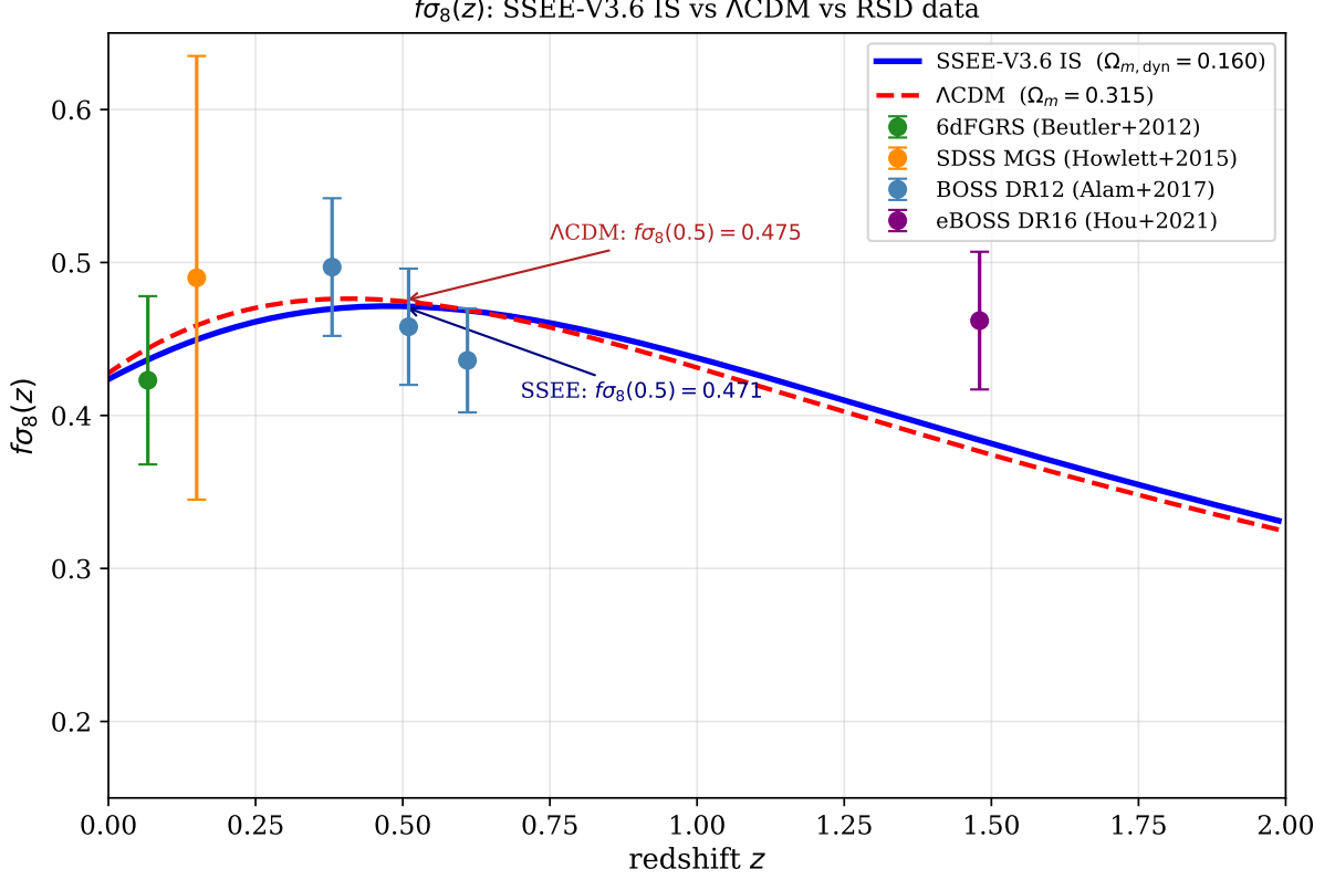
Figure 4: f\sigma_8(z) for SSEE-V3.6 IS (solid blue) and \Lambda CDM (dashed red) versus RSD measurements from 6dFGRS [?], SDSS MGS [?], BOSS DR12 [?], and eBOSS DR16 [?]. The SSEE prediction ( \Omega_{m,\text{cosm}} = 0.30889 in growth equation) is essentially identical to \Lambda CDM at z < 1 , with a mean tension of 0.70\sigma across six data points (vs. 0.73\sigma for \Lambda CDM).
