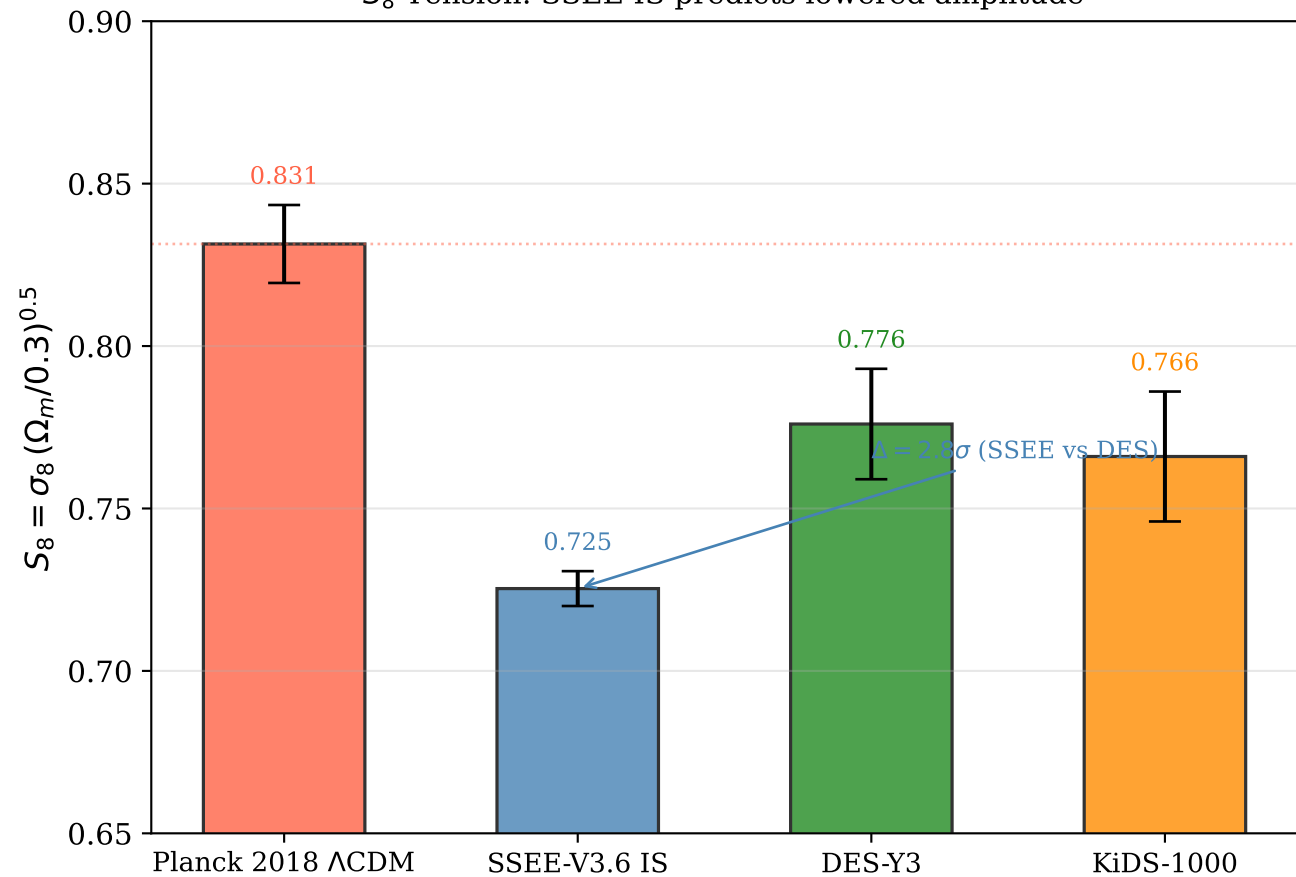
S_8 Tension: SSEE IS predicts lowered amplitude
