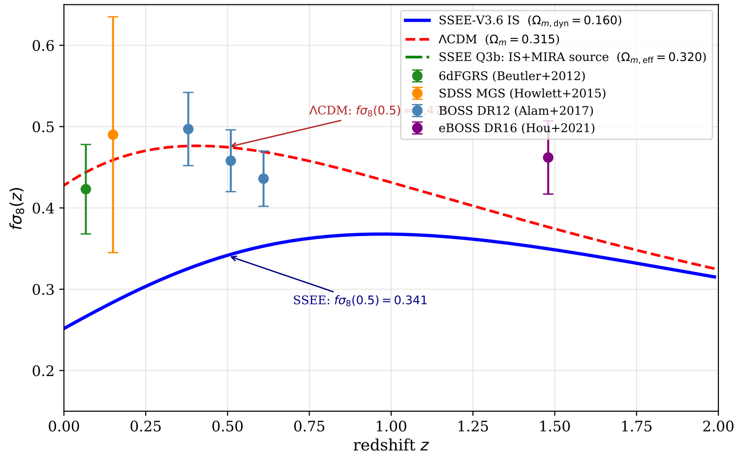
f\sigma_8(z) : SSEE-V3.6 IS vs \Lambda CDM vs RSD data (falsifiable prediction: 28% suppression at z = 0.5 )
