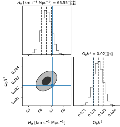
SSEE-V3.6 posterior (MIRA prior, N_{\text{walkers}} \times N_{\text{steps}} = 100 \times 25000 ). Blue lines: MIRA H_0 = 67.068 km/s/Mpc, BBN \Omega_b h^2 = 0.02218 .
