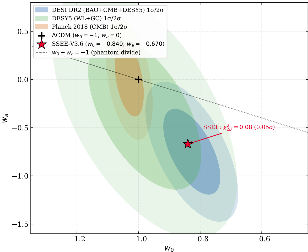
SSEE-V3.6 in the w_0 - w_a plane (DESI DR2 + Planck 2018 + DESY5)
