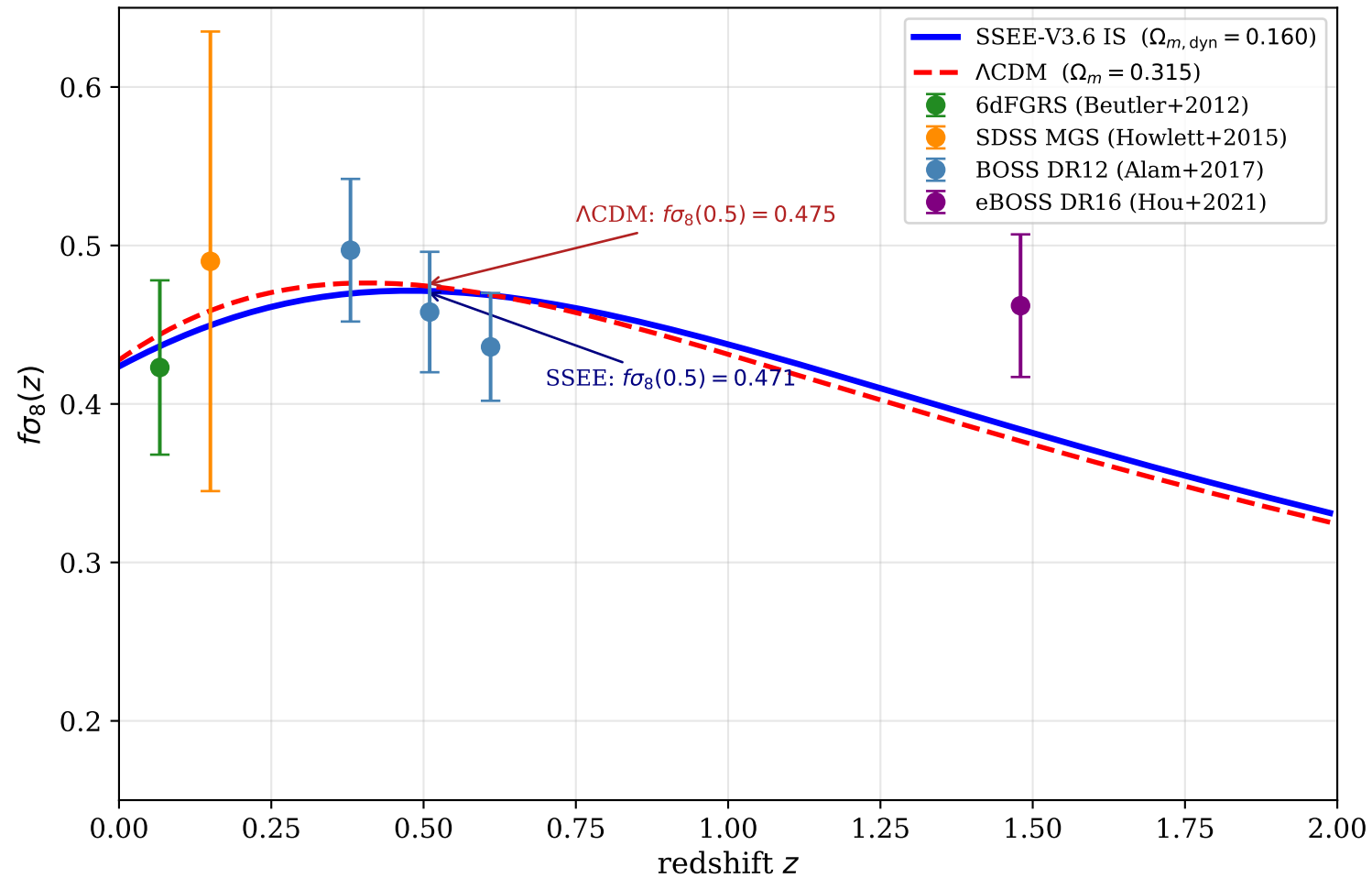
f\sigma_8(z) : SSEE-V3.6 IS vs \Lambda CDM vs RSD data
