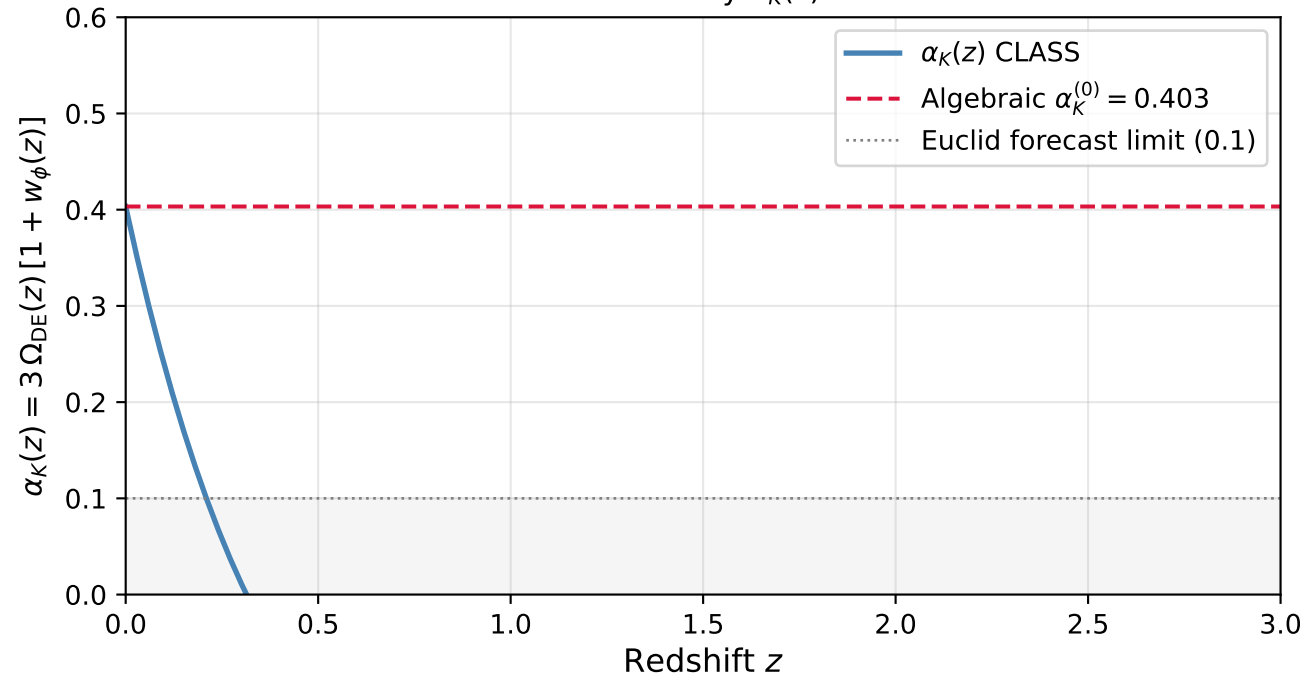
Bellini-Sawicki kinematicity \alpha_K(z) — SSEE-V3.6
