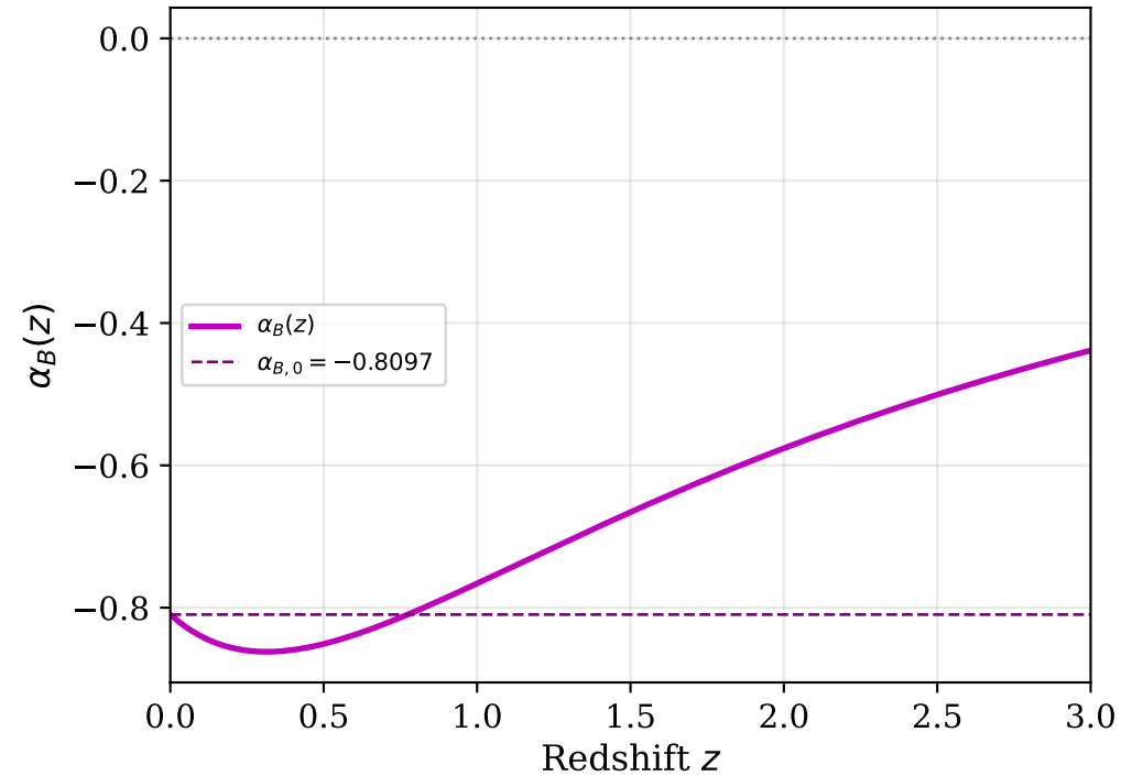
Kinetic Braiding Evolution (tracker)
