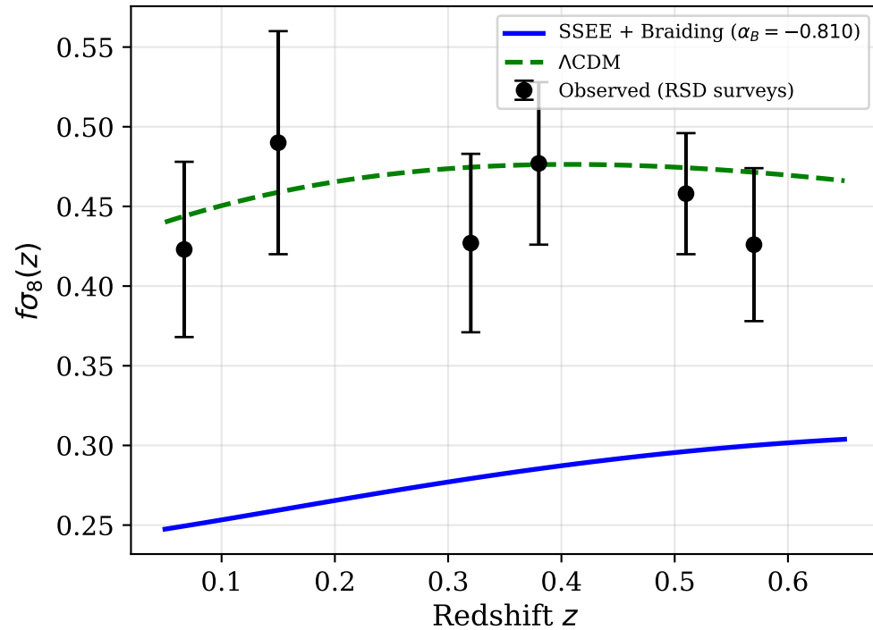
Growth Rate f\sigma_8
